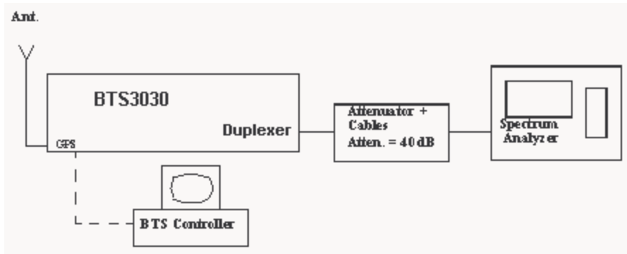
Figure 3 : Test Setup for Occupied Bandwidth Measurement
