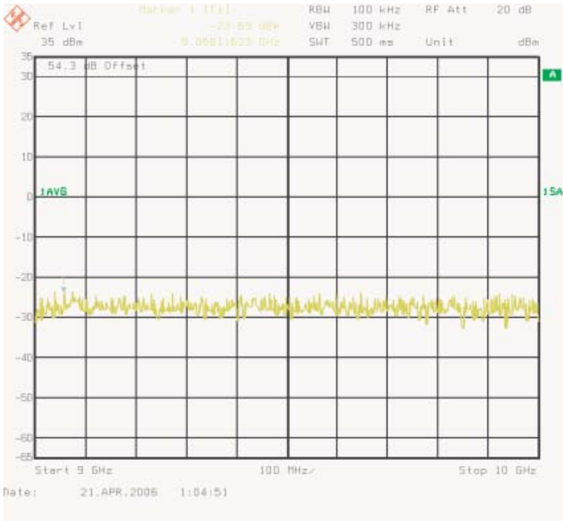
Figure 58 : Three Carriers - A Band Spurious emissions 9000-10000 MHz Ch 226, 267, 308
