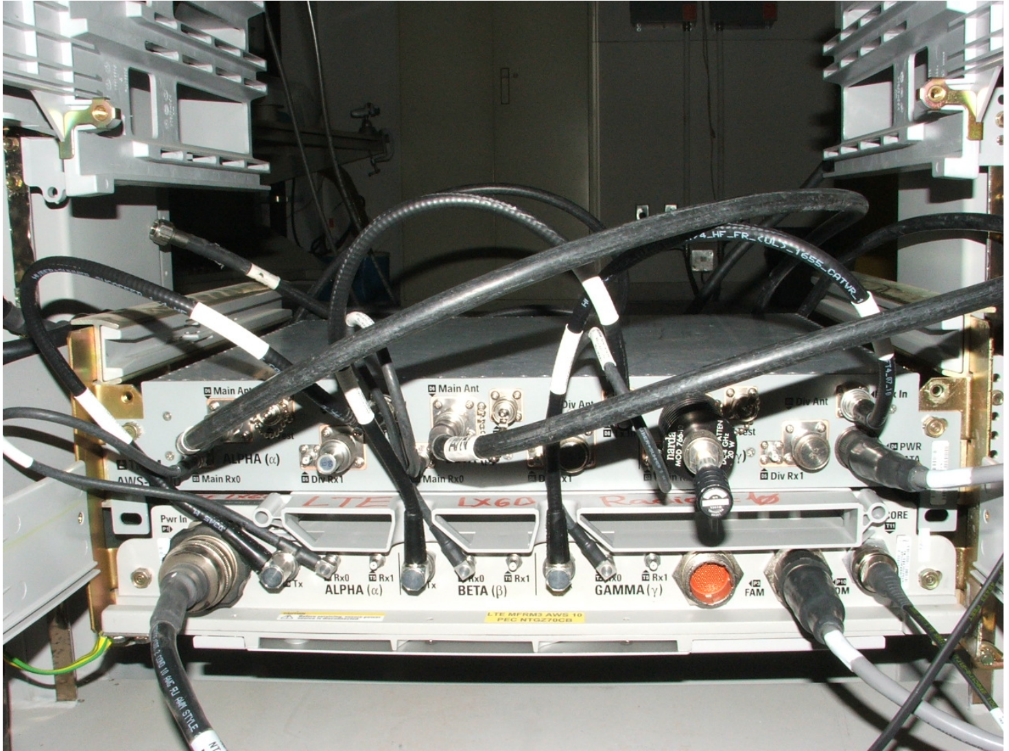
Figure 2. LTE MFRM3 1.7/2.1GHz Assembly Front View. Fan Assembly Removed
