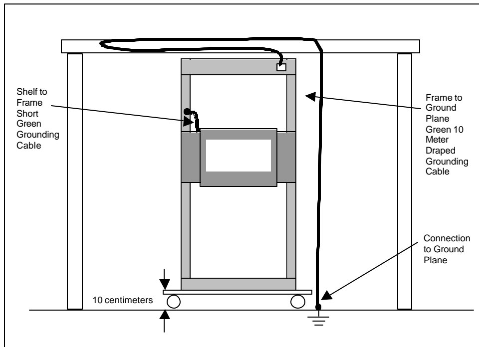
Figure 4-2: System grounding
