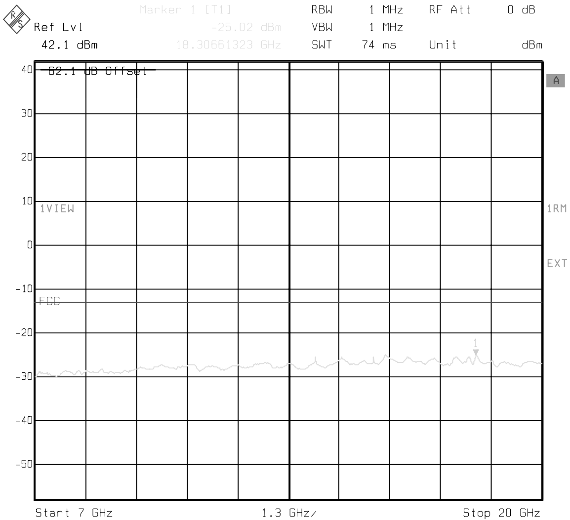
Figure 16 : Conducted Spurious Emissions - 2 Carrier, Channels 650, 675 (7 GHz - 20 GHz)
