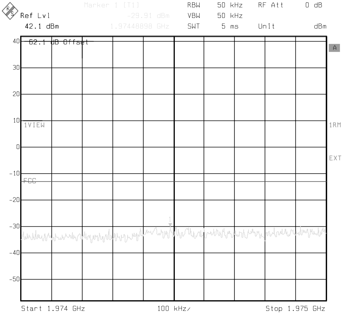
Figure 17 : Conducted Spurious Emissions - 3 Carrier, Channels 925, 950, 975 (Lower adjacent 1 MHz)
