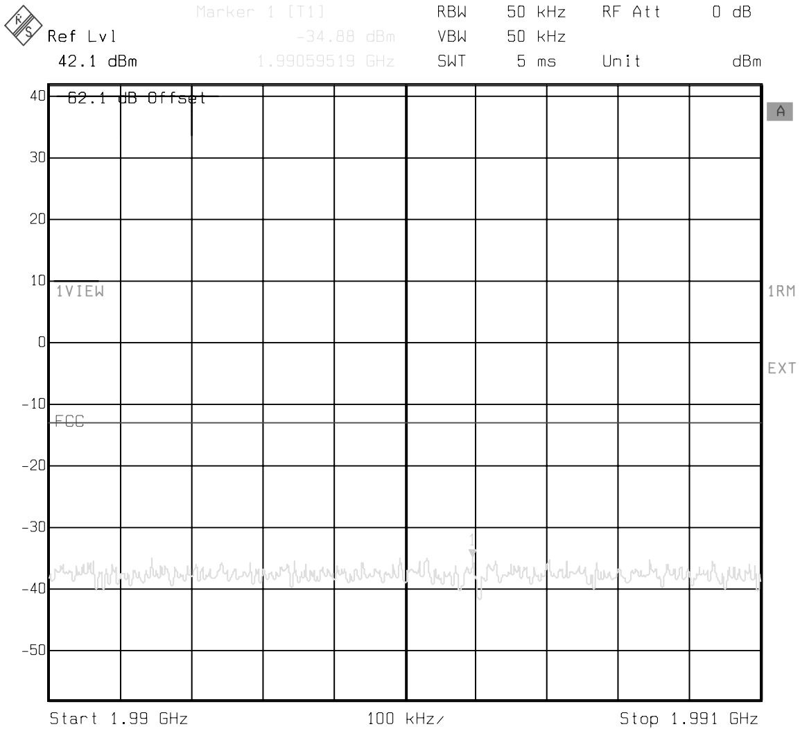
Figure 18 : Conducted Spurious Emissions - 3 Carrier, Channels 925, 950, 975 (Upper adjacent 1 MHz)
