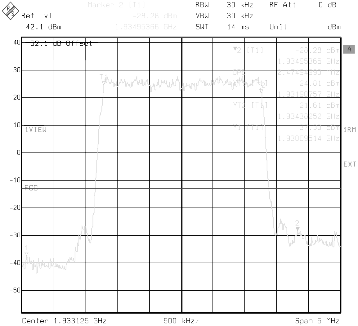
Figure 4 : Occupied Bandwidth - 2 Carrier, Channel 50, 75
