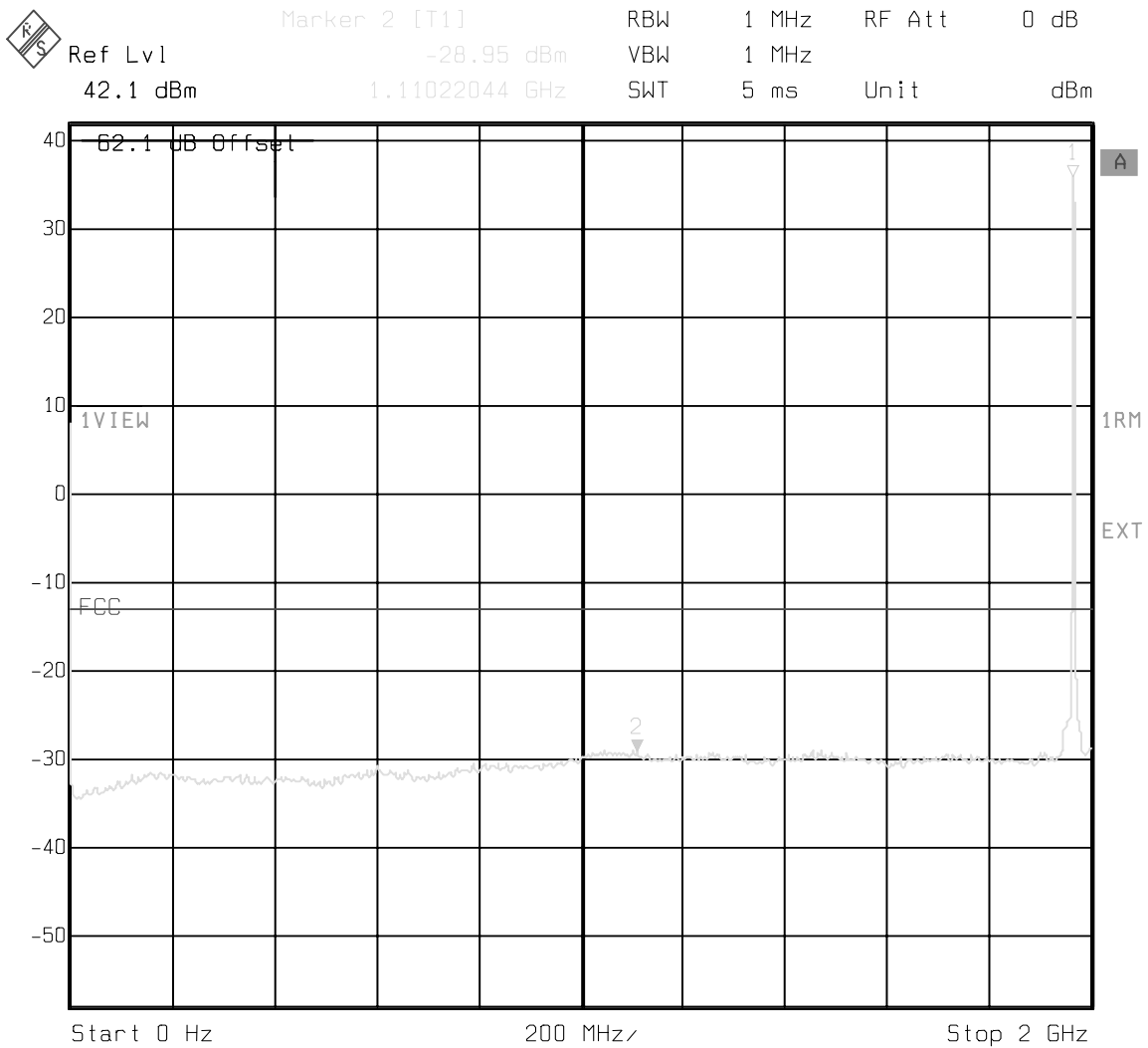
Figure 14 : Conducted Spurious Emissions - 2 Carrier, Channels 650, 675 (10 kHz - 2 GHz)
