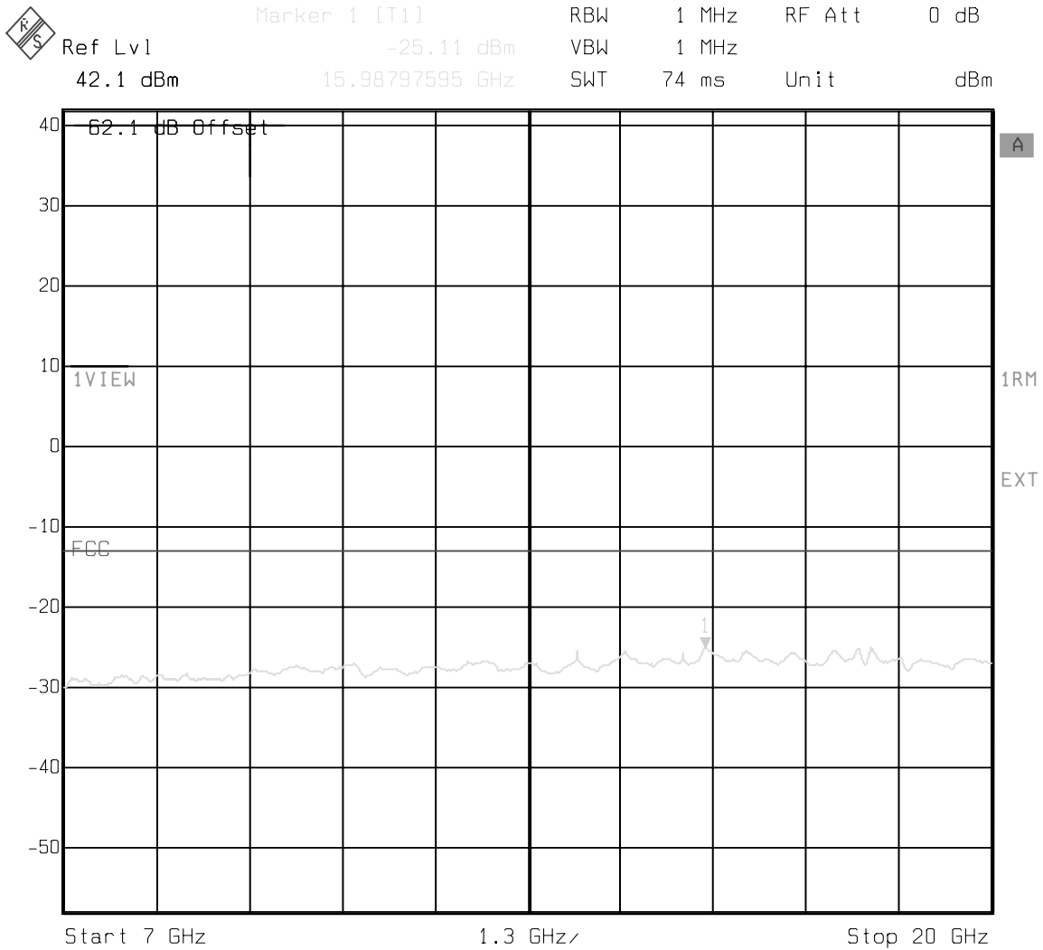
Figure 21 : Conducted Spurious Emissions - 3 Carrier, Channels 925, 950, 975 (7 GHz - 20 GHz)
