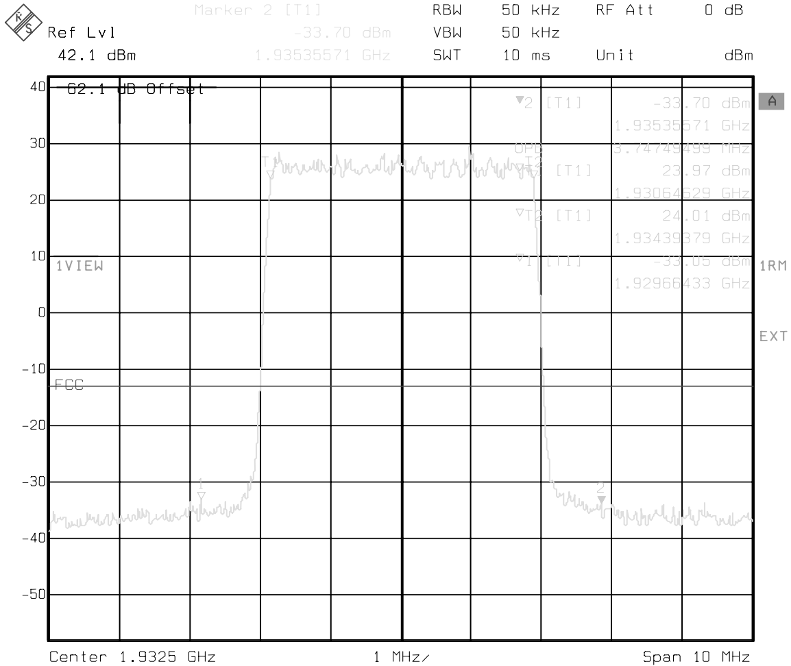
Figure 5 : Occupied Bandwidth - 3 Carrier, Channel 25, 50, 75
