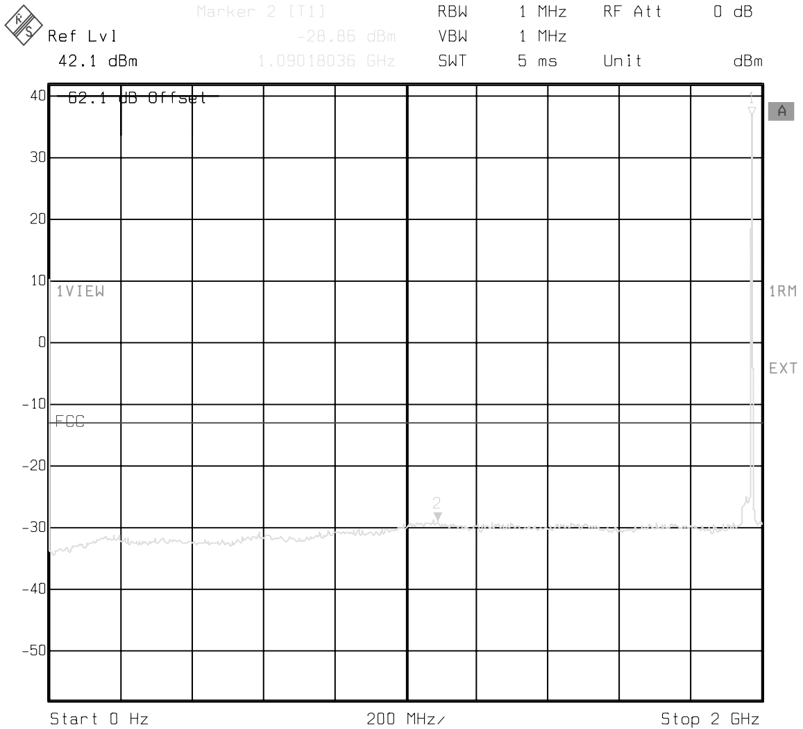
Figure 9 : Conducted Spurious Emissions - 1 Carrier, Channel 775 (10kHz - 2 GHz)
