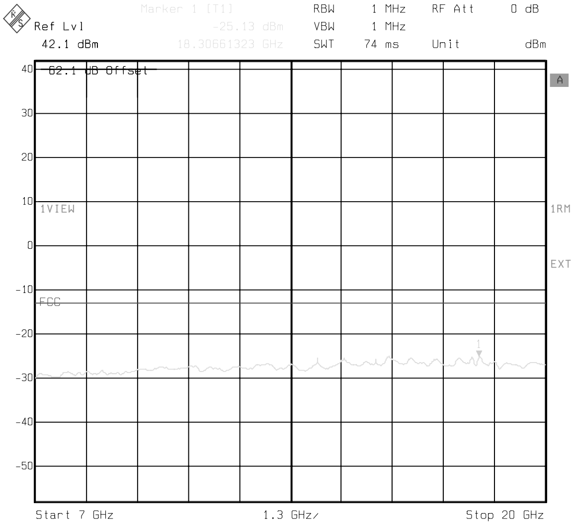
Figure 11 : Conducted Spurious Emissions - 1 Carrier, Channel 775 (7 GHz - 20 GHz)
