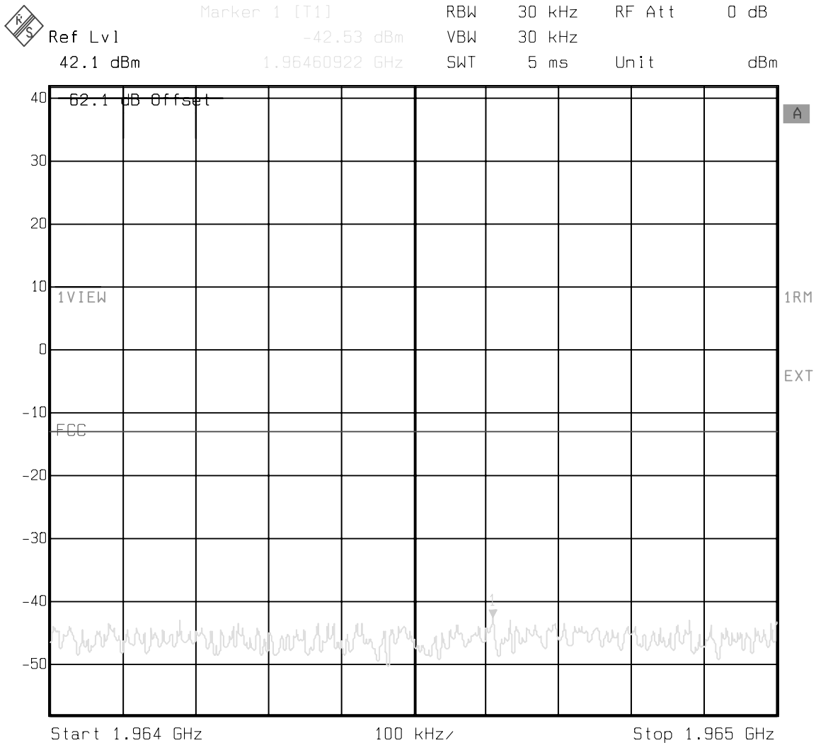
Figure 7 : Conducted Spurious Emissions - 1 Carrier, Channel 775 (Lower adjacent 1 MHz)
