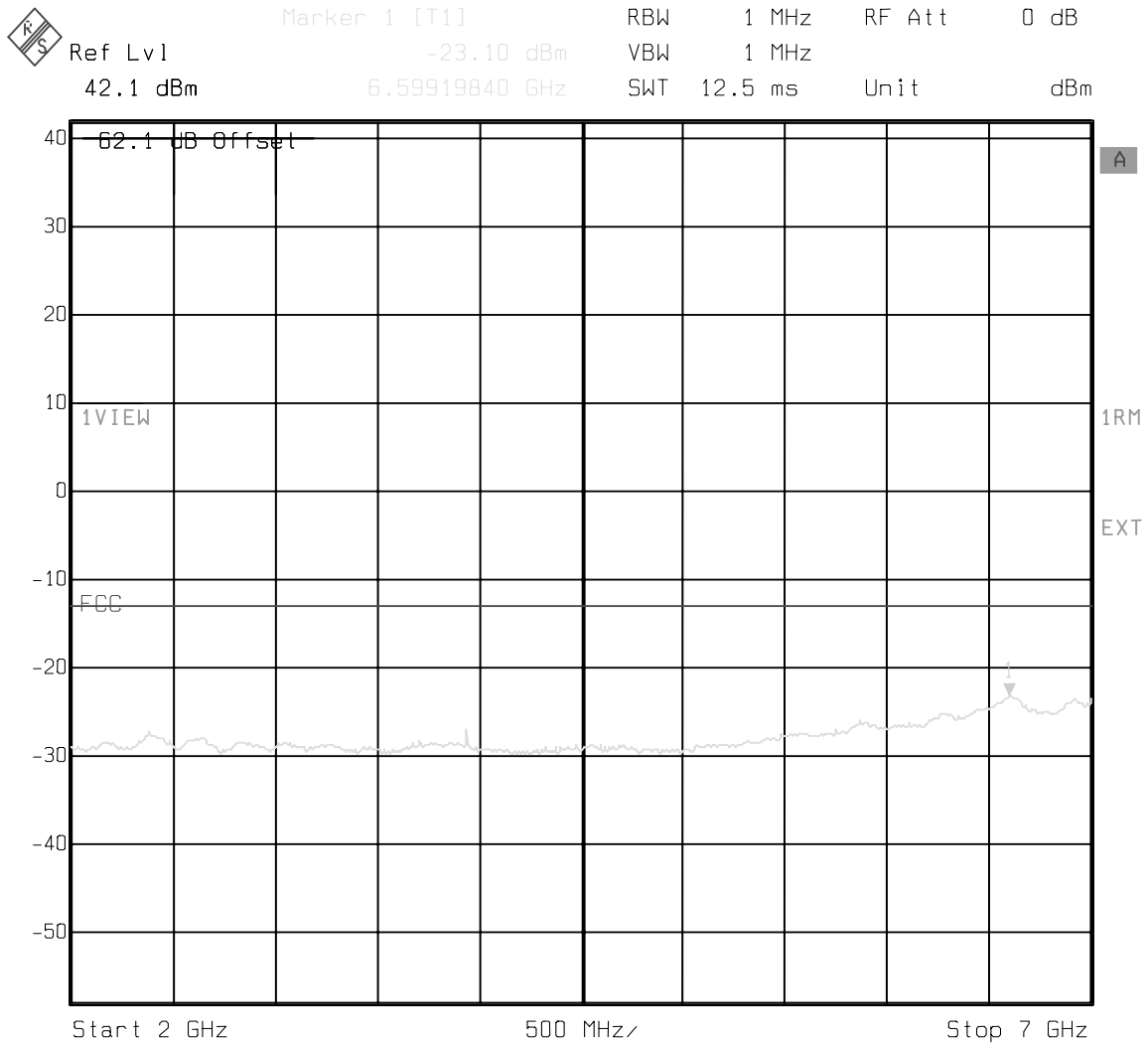
Figure 10 : Conducted Spurious Emissions - 1 Carrier, Channel 775 (2 GHz - 7 GHz)
