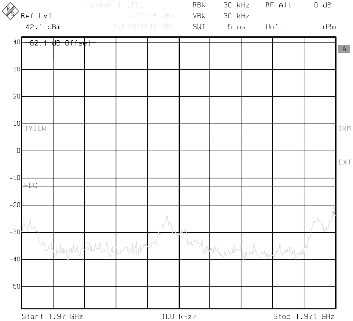
Figure 8 : Conducted Spurious Emissions - 1 Carrier, Channel 775 (Upper adjacent 1 MHz)
