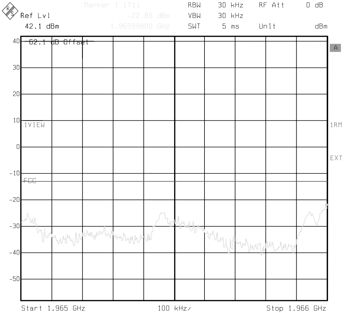
Figure 13 : Conducted Spurious Emissions - 2 Carrier, Channels 650, 675 (Upper adjacent 1 MHz)
