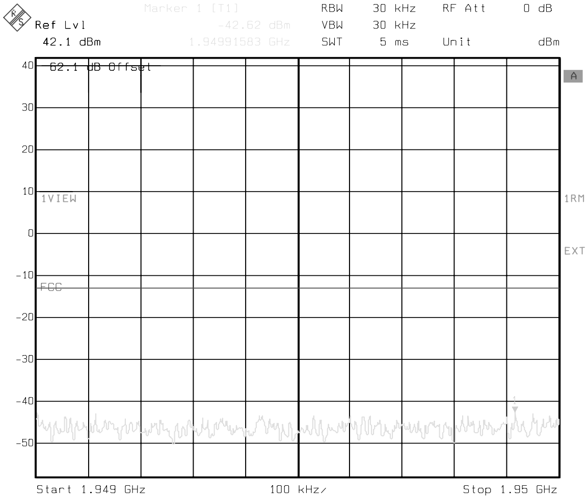
Figure 12 : Conducted Spurious Emissions - 2 Carrier, Channels 650, 675 (Lower adjacent 1 MHz)
