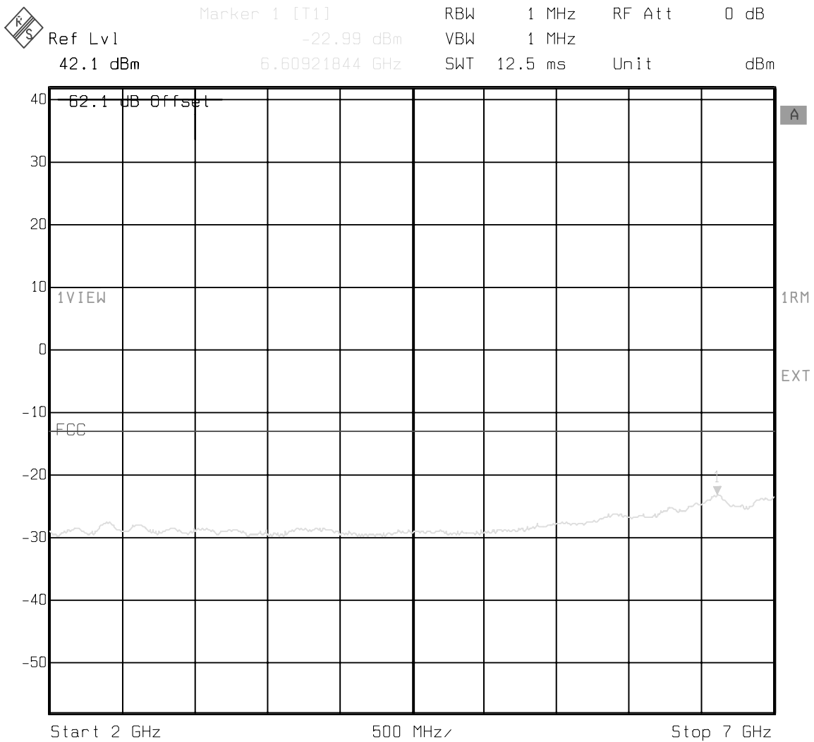
Figure 15 : Conducted Spurious Emissions - 2 Carrier, Channels 650, 675 (2 GHz - 7 GHz)
