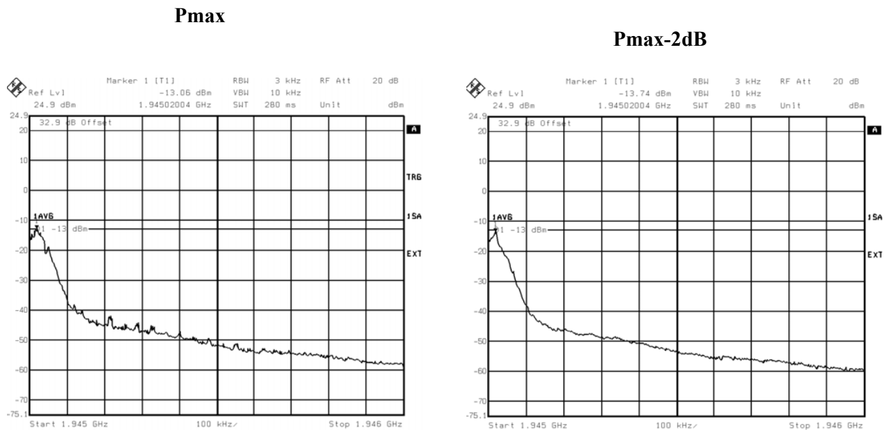
Figure 10 b : +1 MHz adjacent band (Channel 585)
