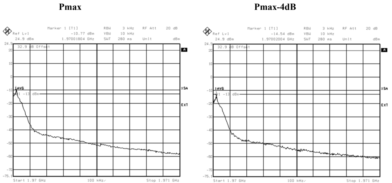
Figure 11 b : +1 MHz adjacent band (Channel 710)
