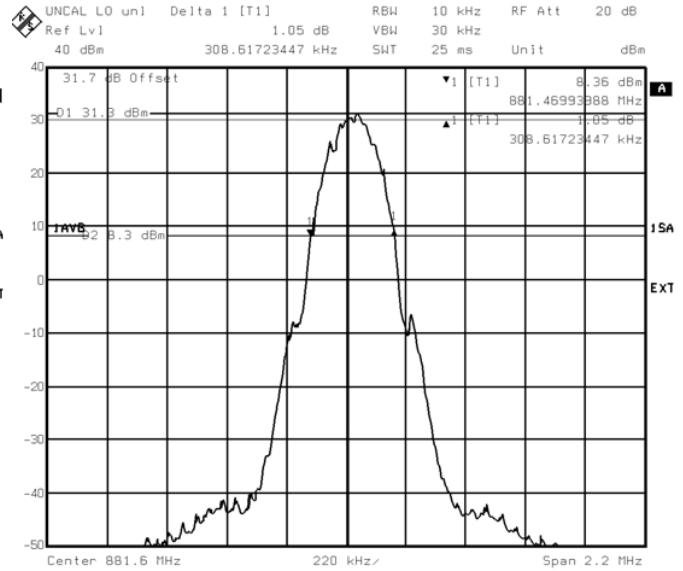
Figure 2: sample plot for occupied bandwidth, @ M (GSM 850 band)
