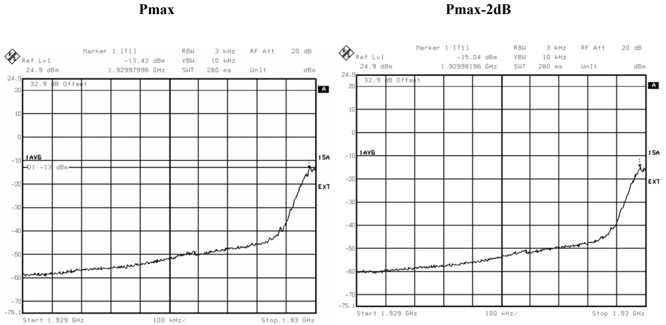
Figure 10 b : +1 MHz adjacent band (Channel 585)
