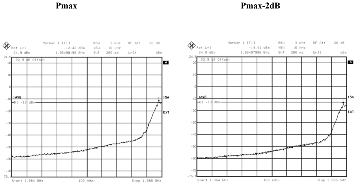
Figure 11 a : -1 MHz adjacent band (Channel 687)
