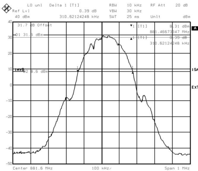
Figure 2: sample plot for occupied bandwidth, @ M (GSM 850 band)
