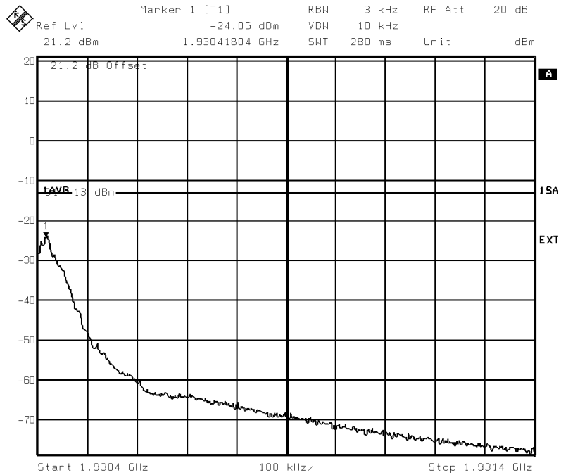
Figure 8 : +1 MHz adjacent band (TDMA1, Channel 512, Pmax)
