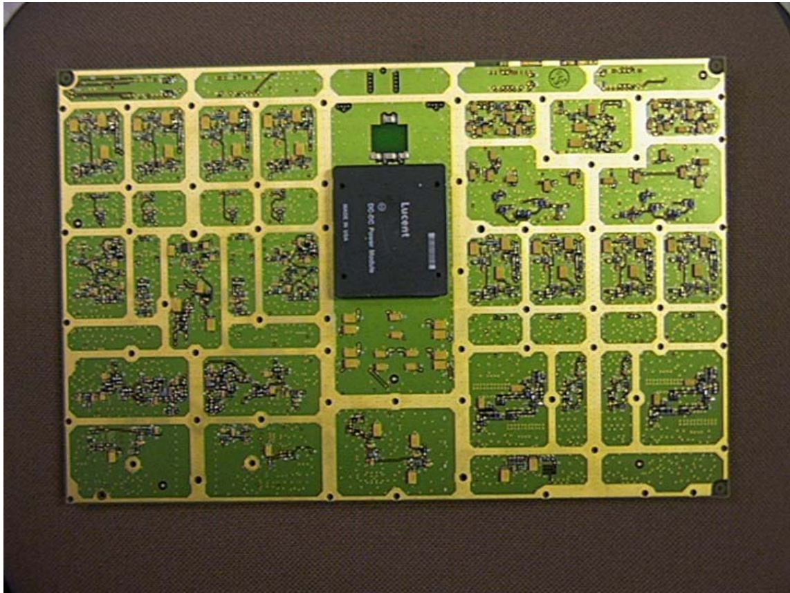
Figure 1: Transceiver PCB (Bottom view)
