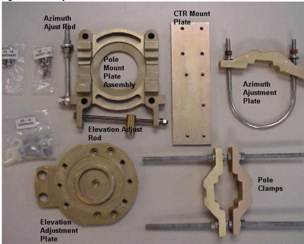
Figure 7 – Fine Adjust Mount
