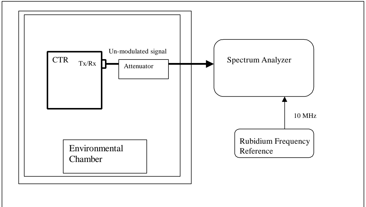
Figure 4: Test Configuration for Radio Frequency Tolerance Test Case
