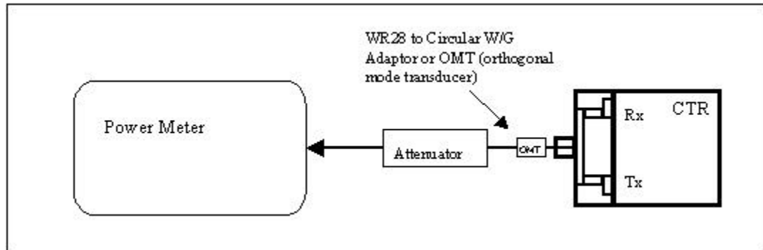
Figure 3: Test Configuration for Tx Output Power, Tx Nominal Output Power
