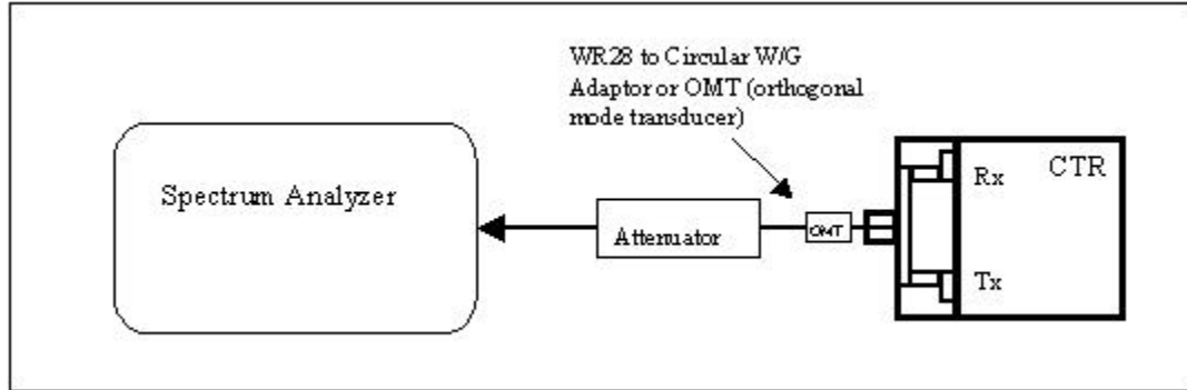
Figure 5: Test Configuration for Spectrum Mask, Occupied Bandwidth, and Spurious Emissions Test Cases
