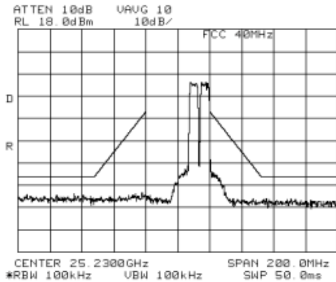
Fig. A-8 (Spectrum Mask, 4QAM, channel T, 2 carriers)
