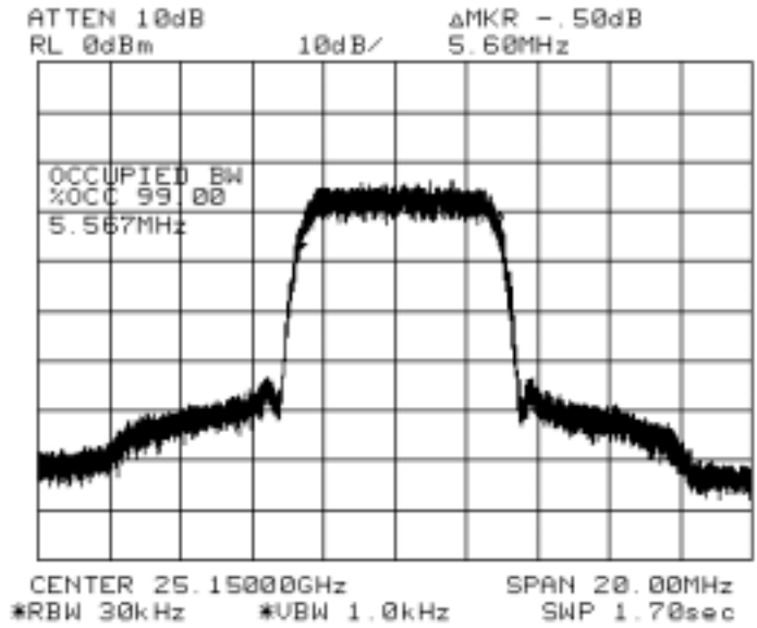
Fig. A-1 (99% Occupied Bandwidth, 1 carrier, 4QAM)
