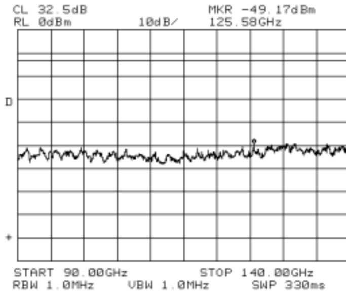
Fig. A-32 (Conducted Spurious Emissions, 16QAM, 1 carrier, 90 – 140GHz)
