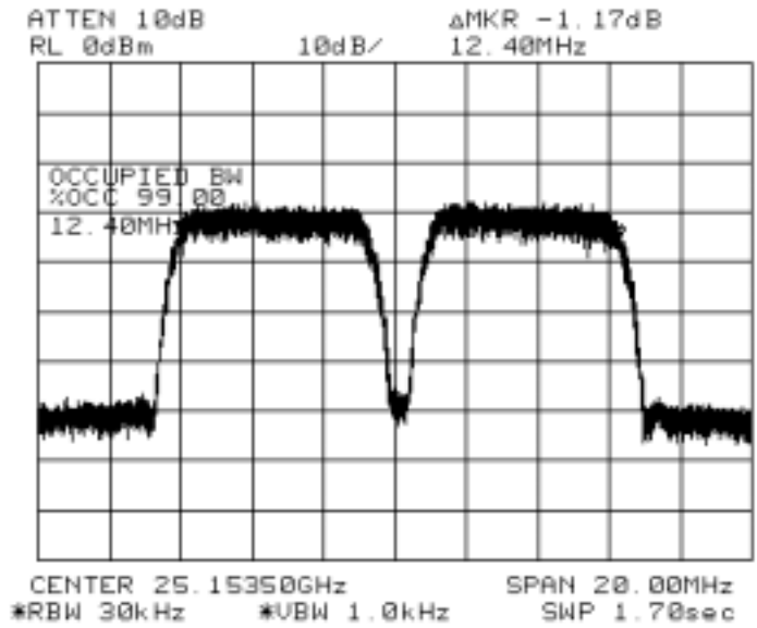
Fig. A-2 (99% Occupied Bandwidth, 2 carriers, 4QAM)
