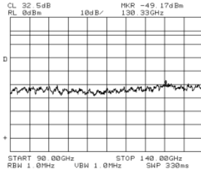
Fig. A-26 (Conducted Spurious Emissions, 4QAM, 2 carriers, 90 – 140GHz)
