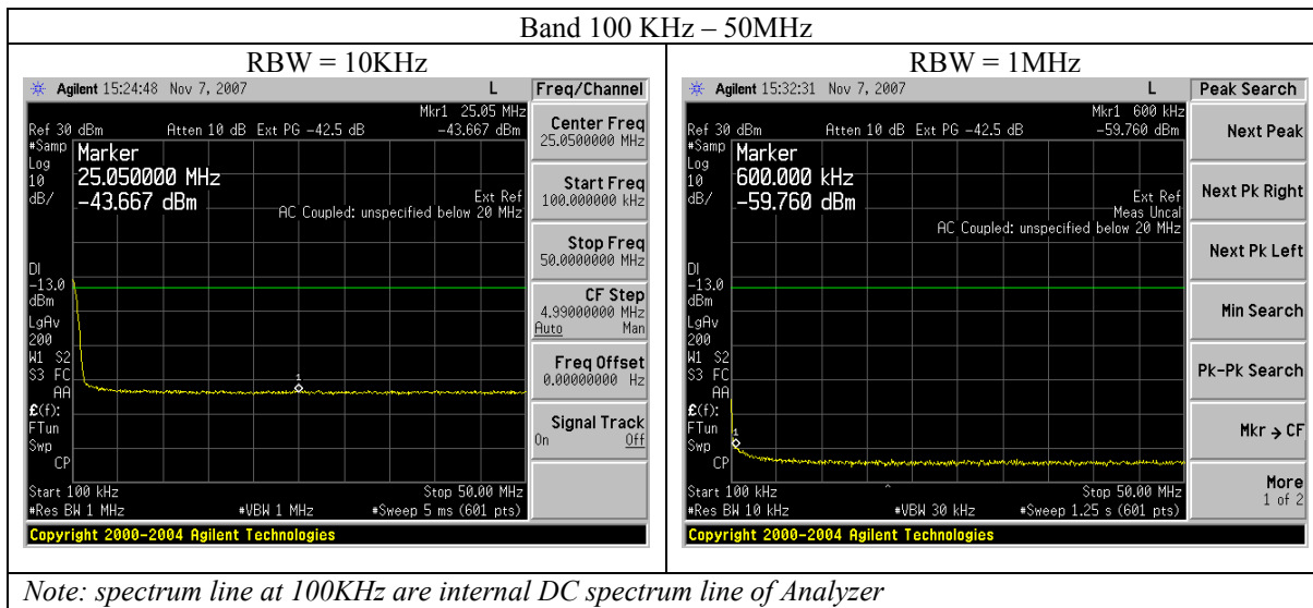
Figure: Out of block emission (Channel 189, Pmax) 8PSK Modulation – HD Configuration
