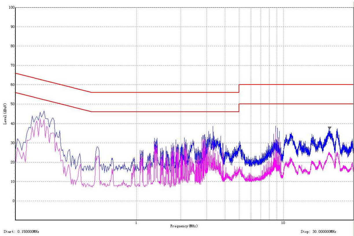
DC port conducted Emission Graph (0V terminal)
