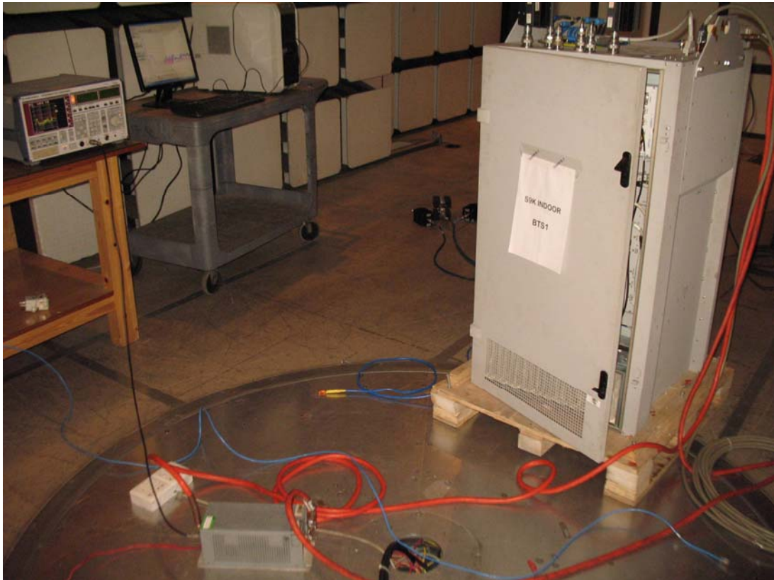
DC port Conducted Emission Test Set-up
