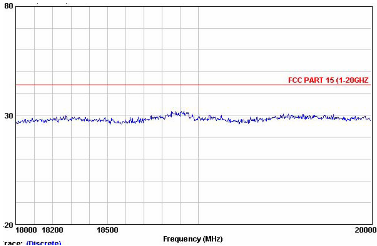
Vertical Radiated Emission Plot (Peak, Max Hold Mode) 18-20GHz
