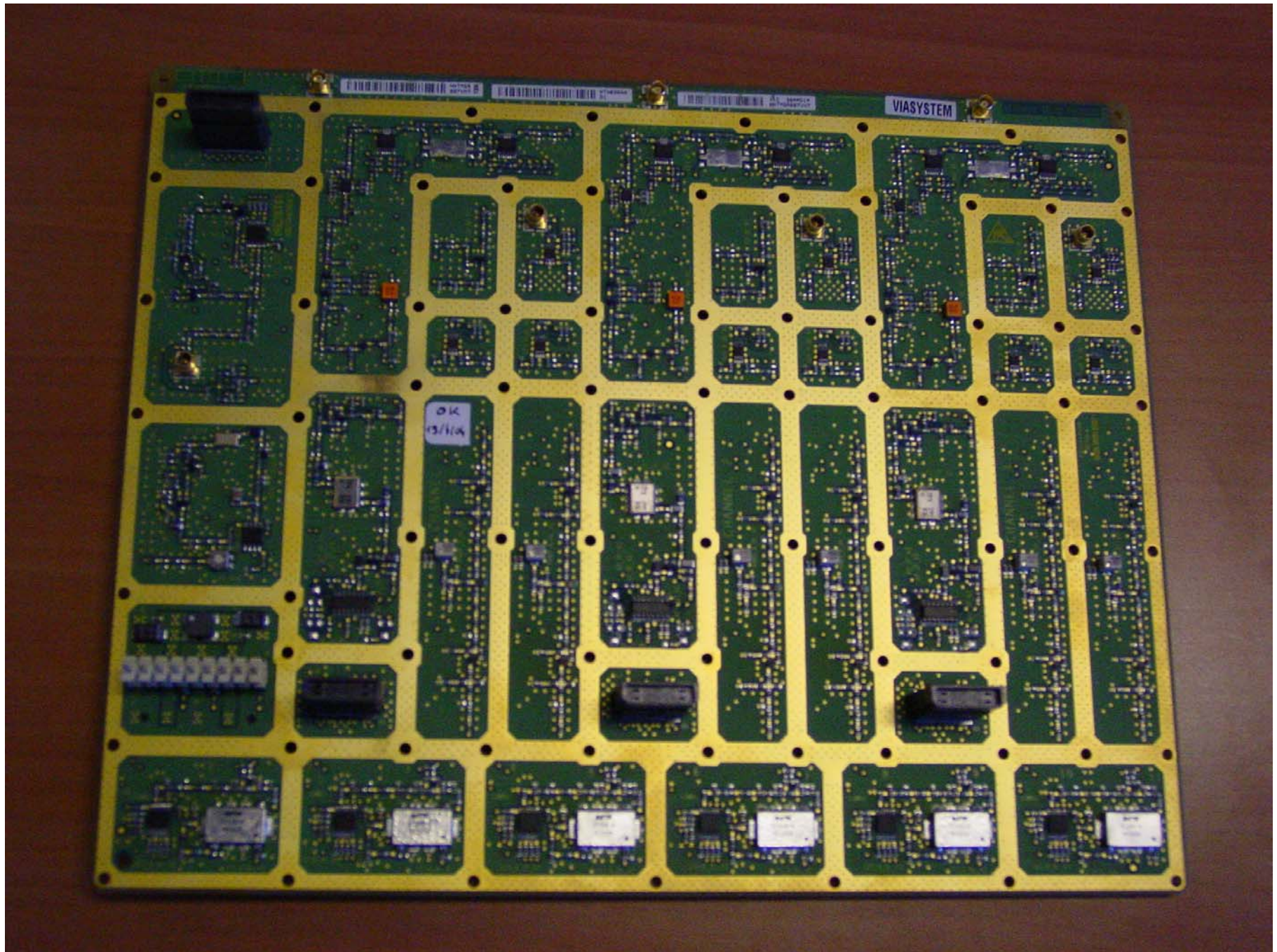
MRM Radio part: TX board (Top)
