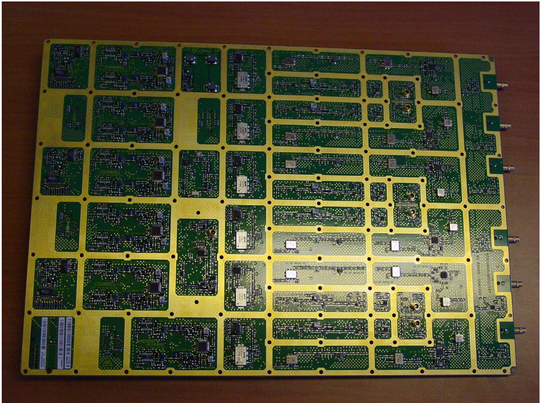
MRM Radio part: RX board (Bottom)
