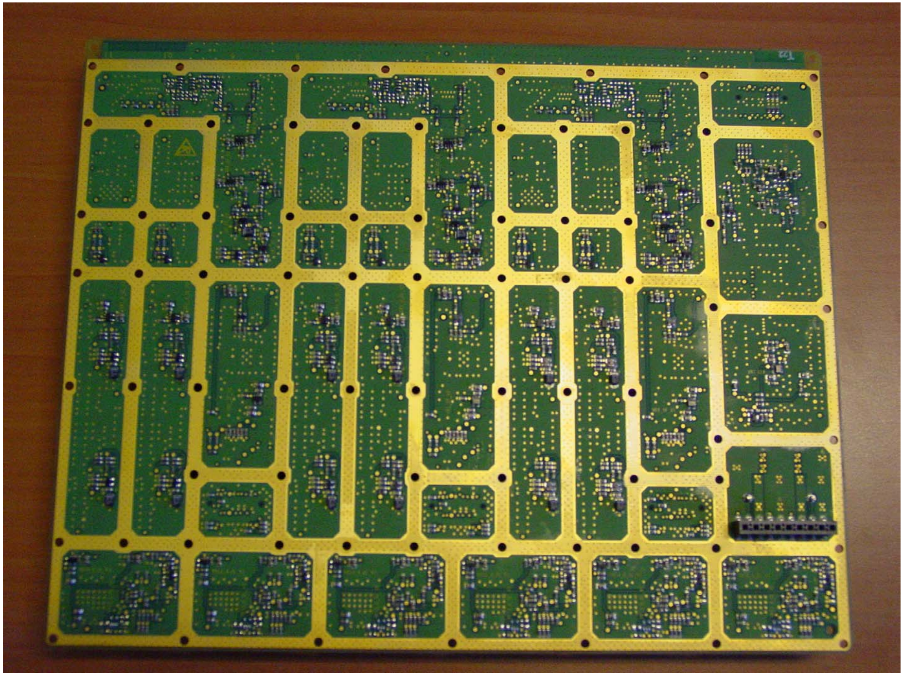
MRM Radio part: TX board (Bottom)
