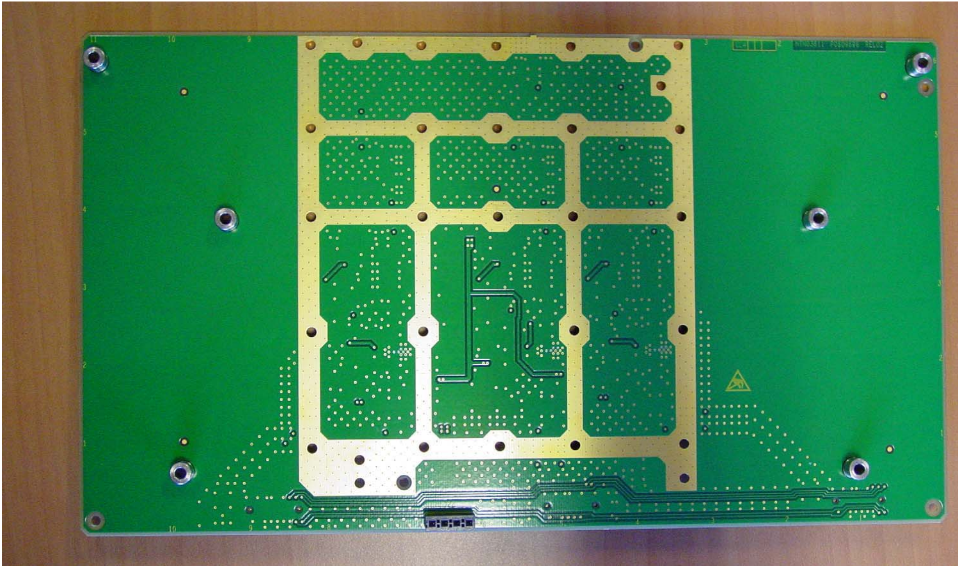
MRM Radio part: TX Booster board (Bottom)
