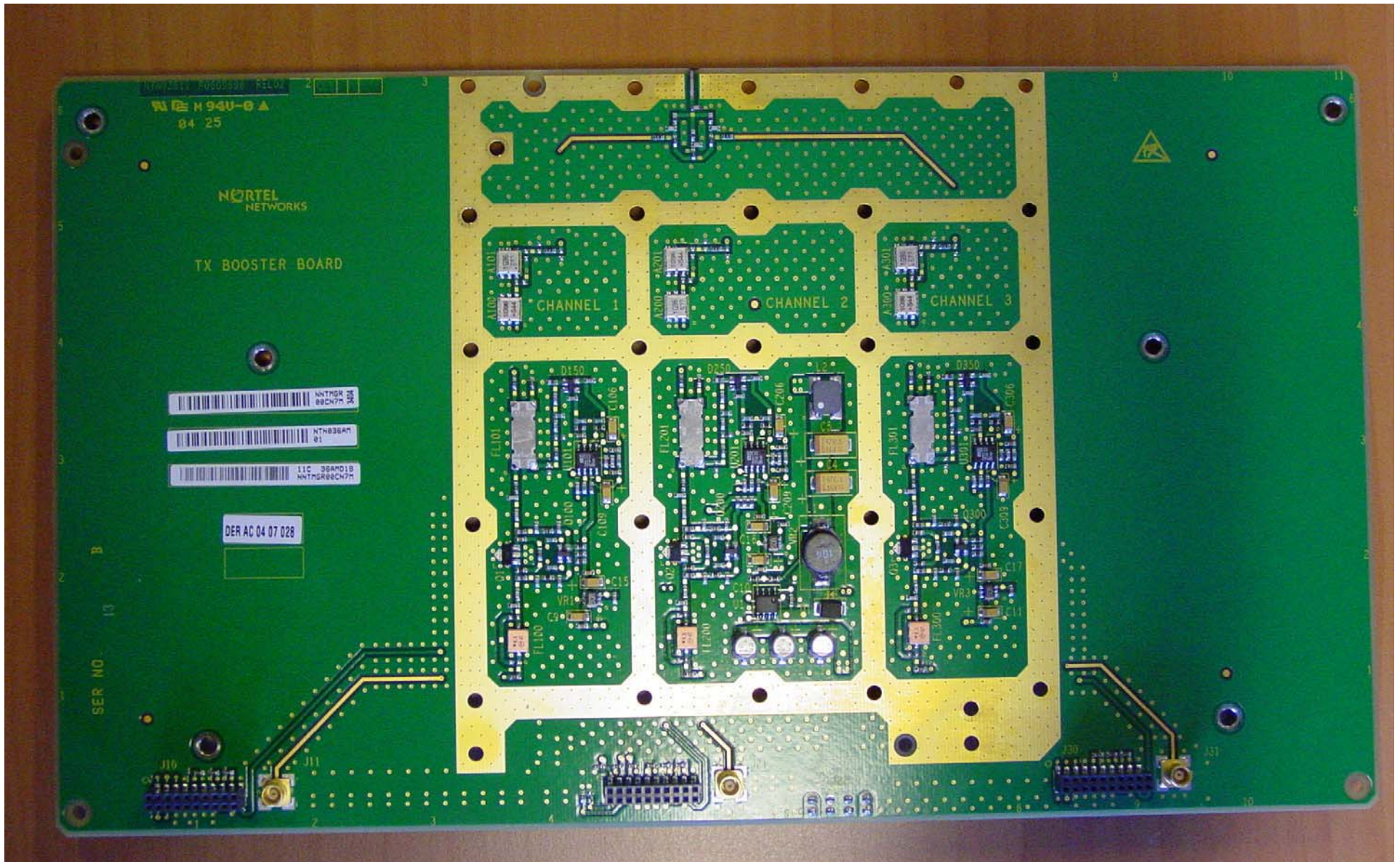
MRM Radio part: TX Booster board (Top)
