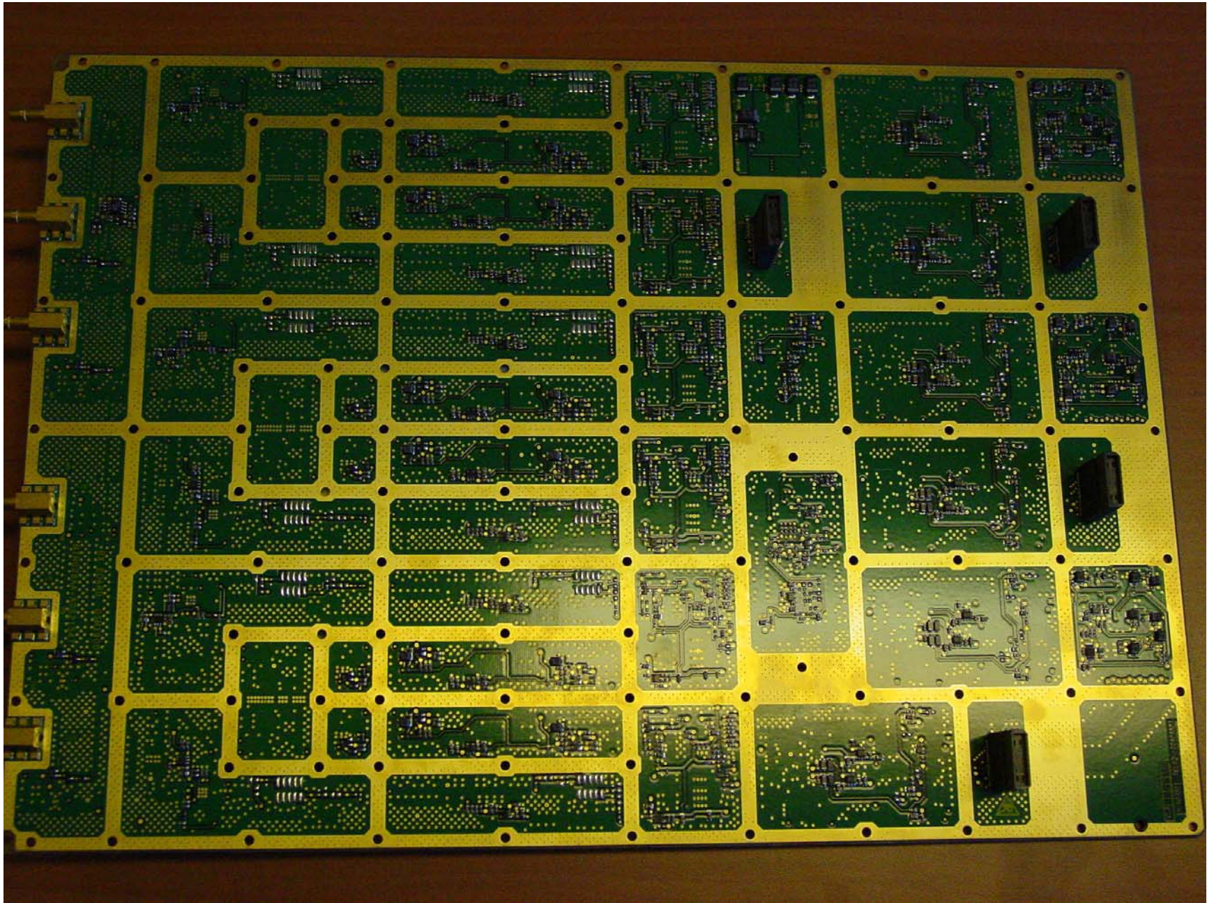
MRM Radio part: RX board (Top)
