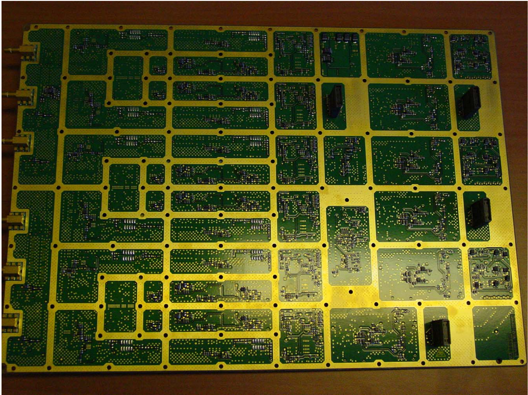
RM Radio part: RX board (Top)
