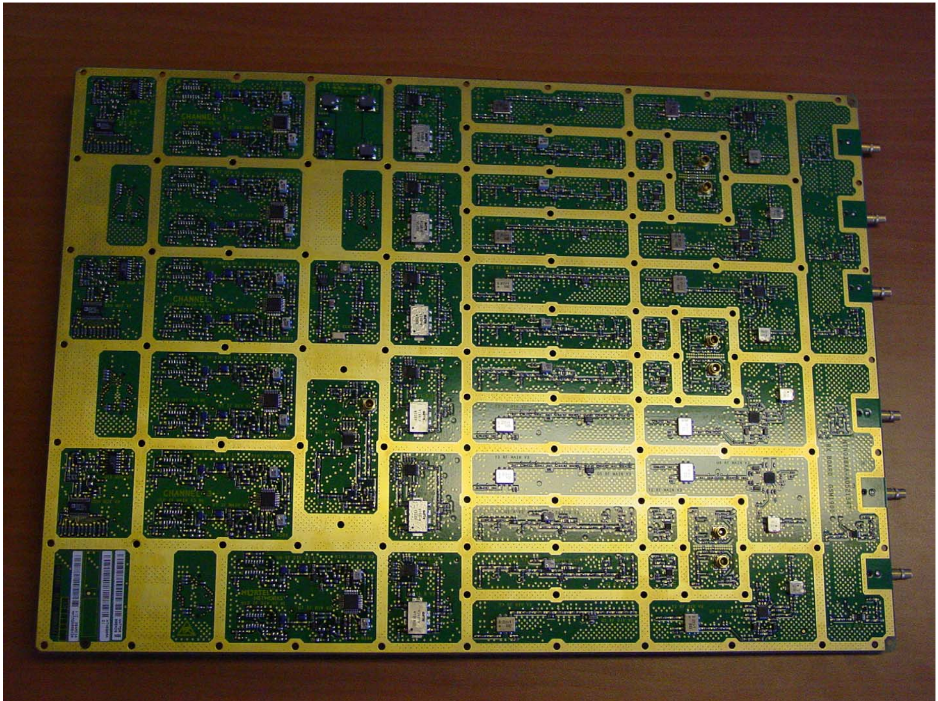
RM Radio part: RX board (Bottom)
