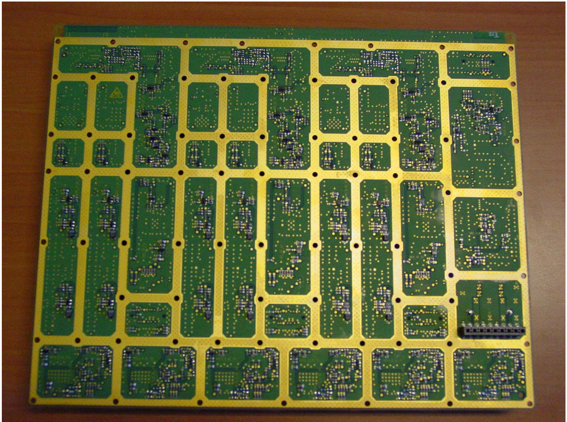
RM Radio part: TX board (Bottom)
