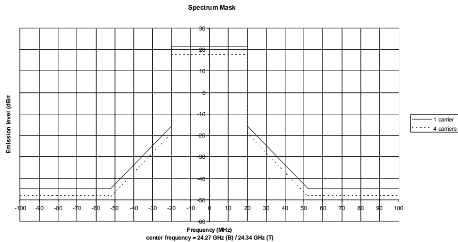
Fig. 5-1: Spectrum Mask limit
