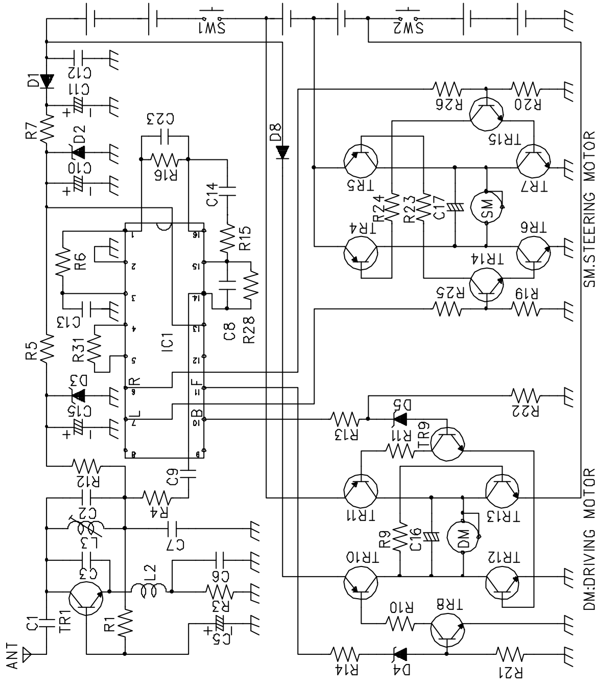
NO.RP7300P CIRCUIT DIAGRAM
