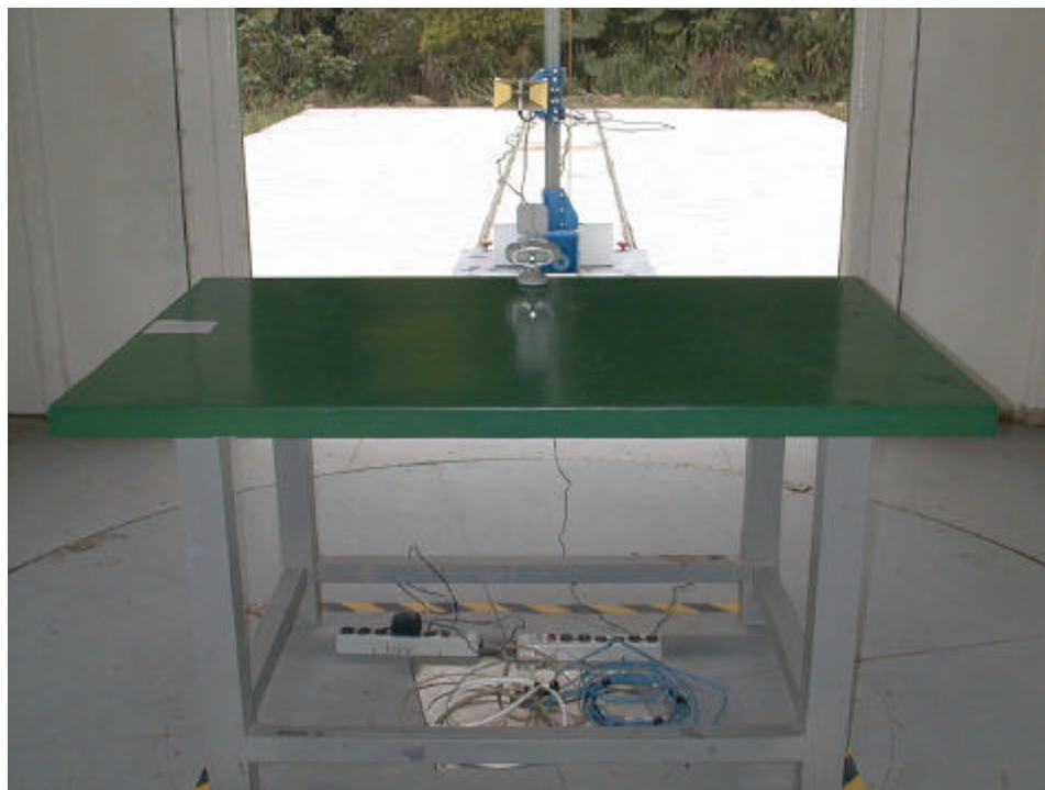
Front View of Radiated Test (Mode 3)
