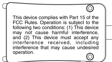
Head band (Right) FCC Part 15 (Engraving) Text size: 6 pt scale 1:1
