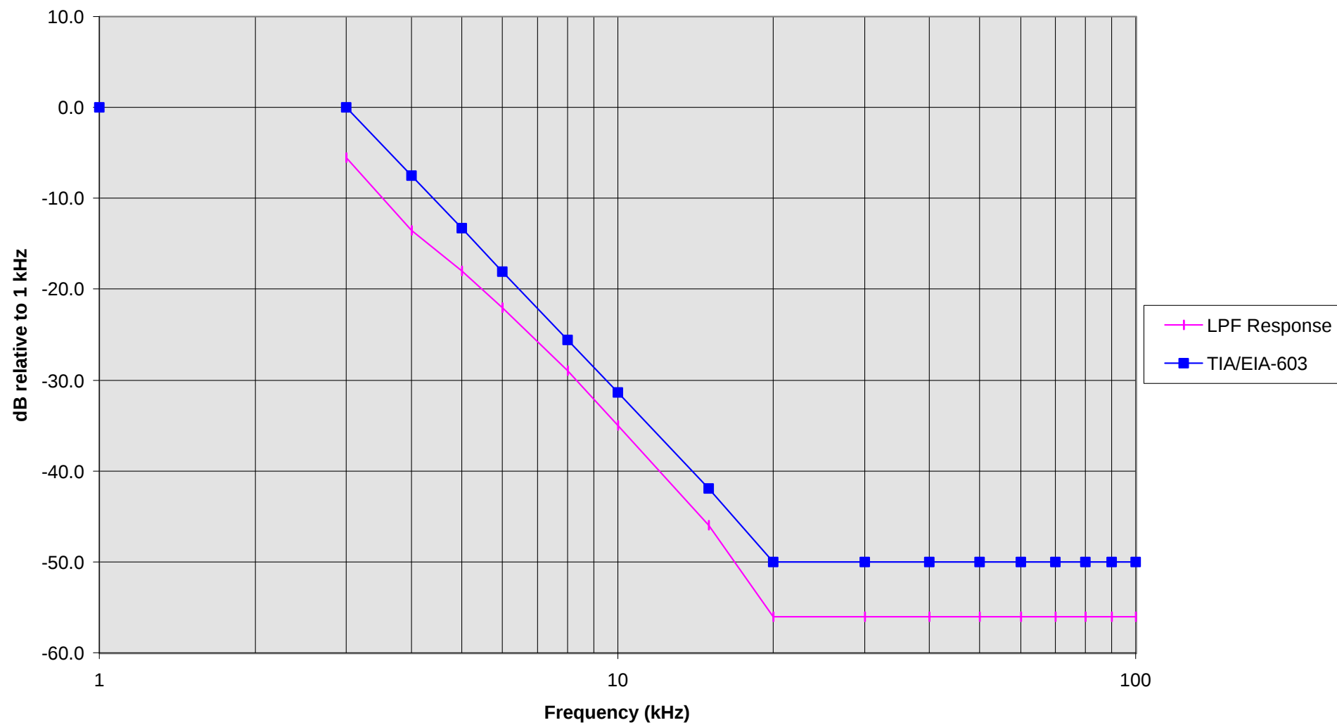
Audio Low Pass Filter Response (Model: 21-1864)
