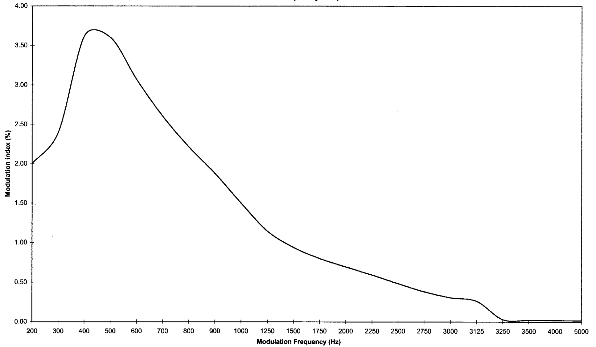
Modulation Frequency Response
