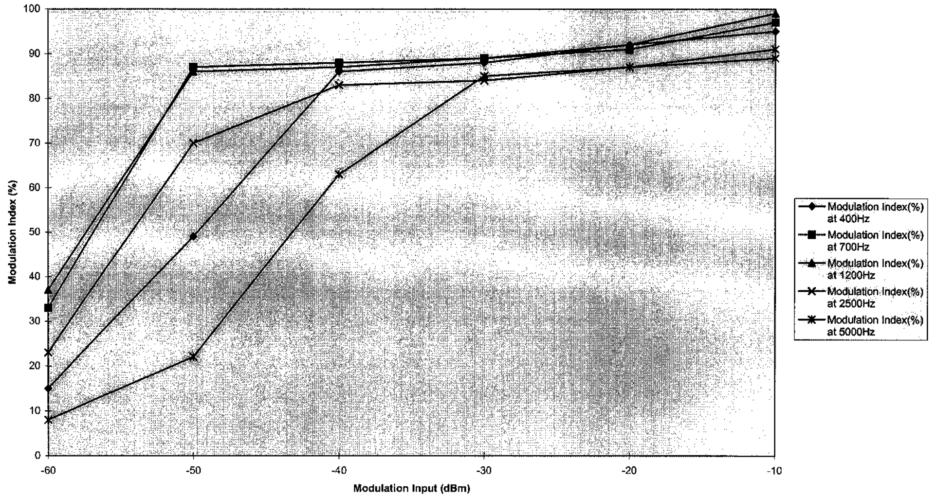
Modulation Limiting Characteristic
