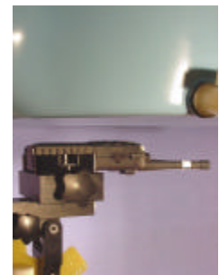
Face-Held SAR Test Setup 2.5cm Separation Distance
