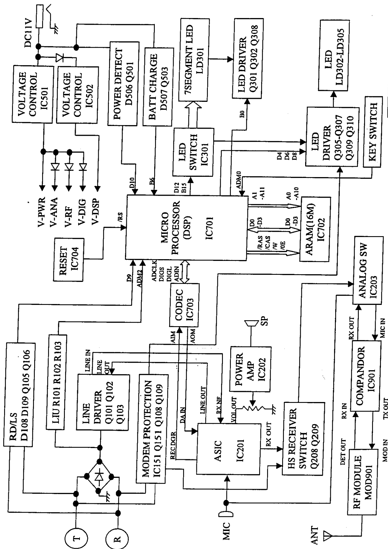
TC-925(TP-3454) BASE BLOCK DIAGRAM
