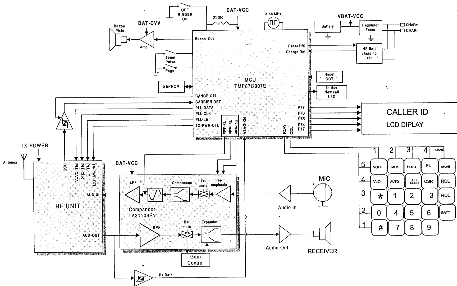
CP-750 Handset Block Diagram
