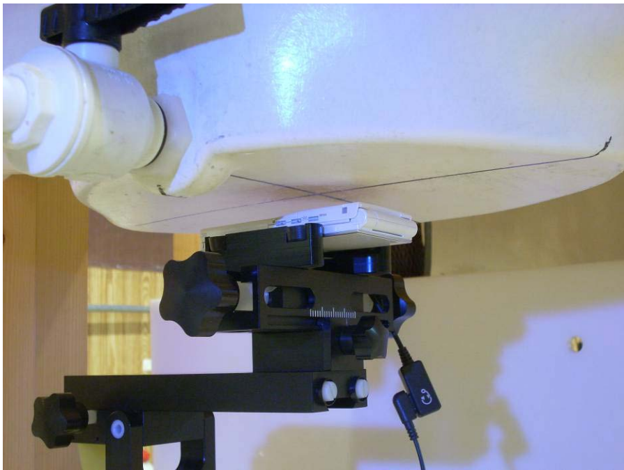
Figure 19-5 SAR Test Photo Setup Photo 5
