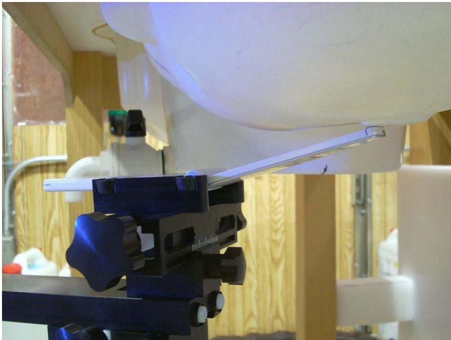
Figure 19-3 SAR Test Photo Setup Photo 4
