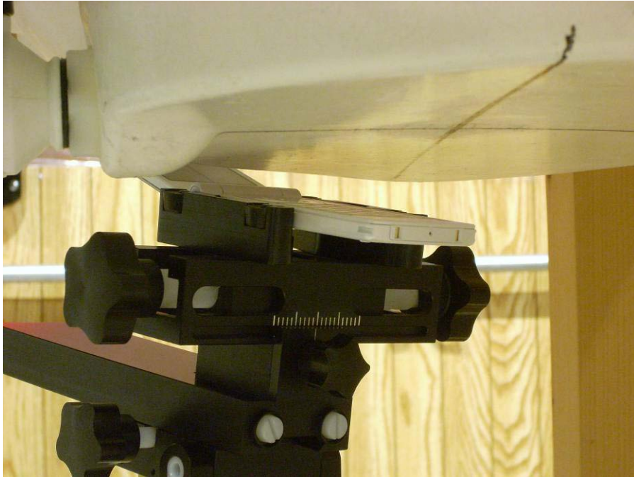
Figure 19-4 SAR Test Photo Setup Photo 5
