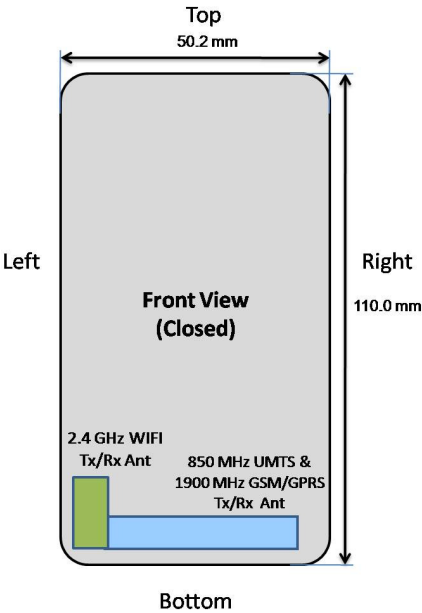
Figure 1-1 DUT Antenna Locations
