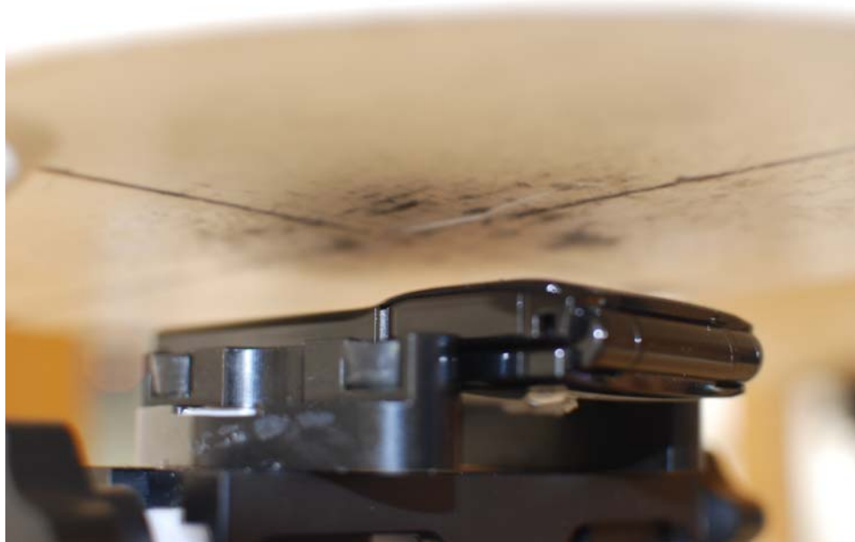
SAR Test Setup Photo 6: Body-Worn at 15mm
