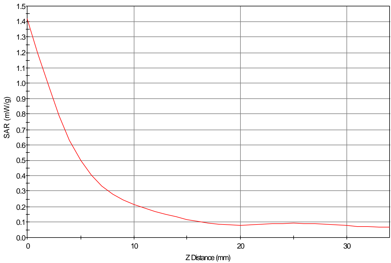
SAR - Z Axis at Hotspot x:73.0 y:-4.0
