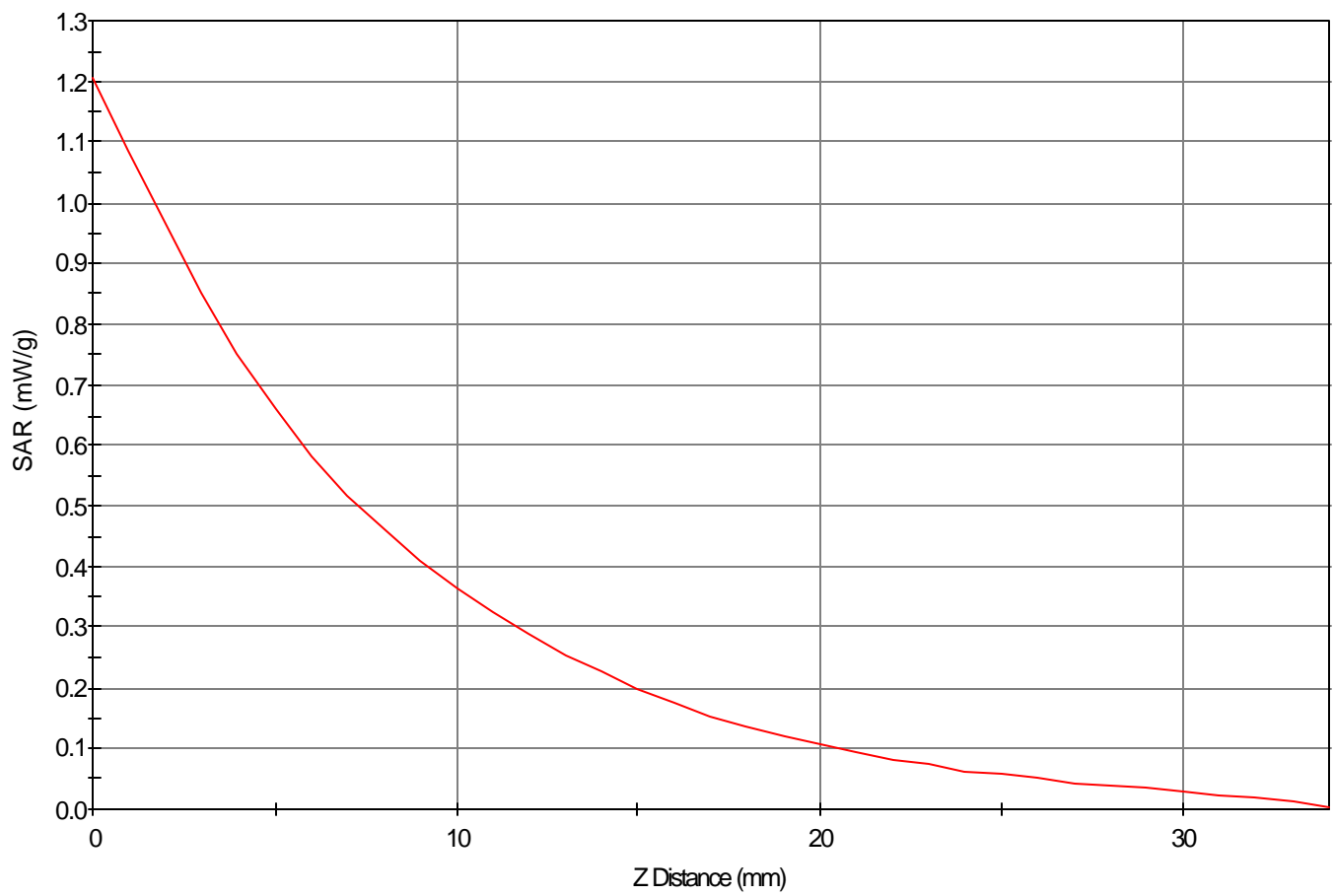
SAR - Z Axis at Hotspot x:61.0 y:3.0
