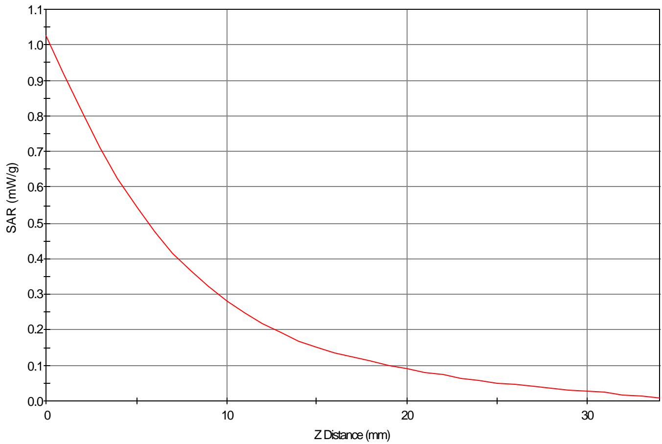
SAR - Z Axis at Hotspot x:57.0 y:10.0
