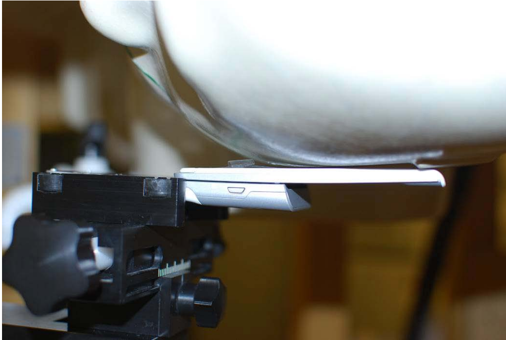
Figure 20-7 SAR Test Setup Photo 7
