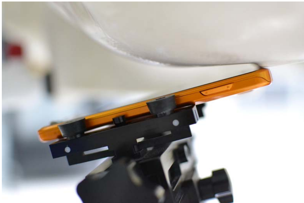
SAR Test Setup 4 - Left Tilt
