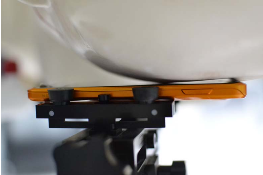
SAR Test Setup 3 - Left Cheek
