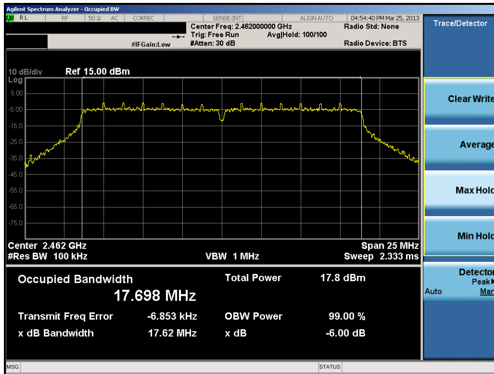
Plot 6-12. 6dB Bandwidth Plot (802.11n (2.4GHz – 800ns GI) – Ch. 11)
