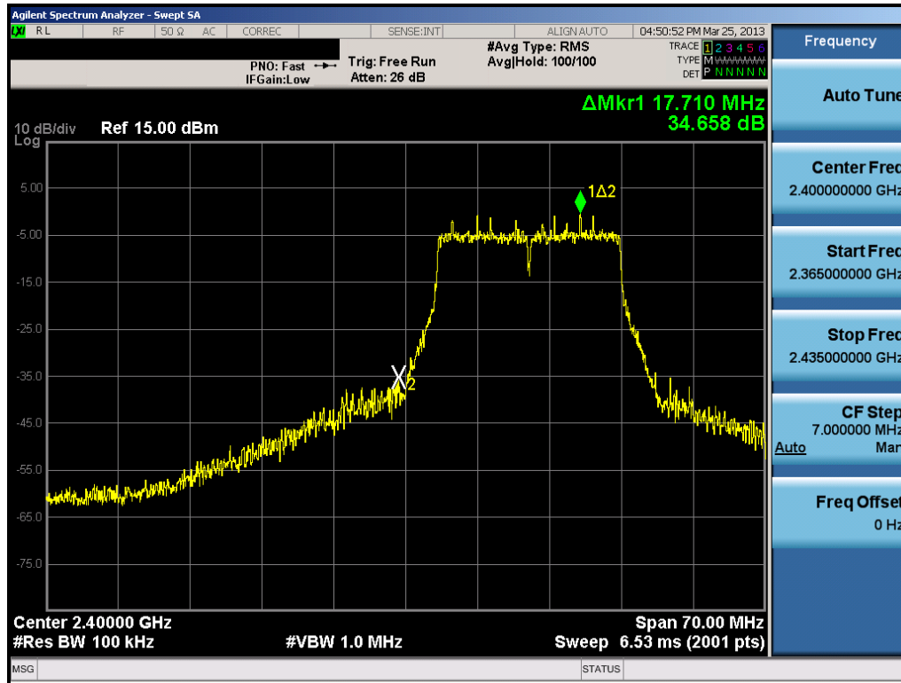
Plot 6-31. Band Edge Plot (802.11n (2.4GHz – 800ns GI) – Ch. 1)
