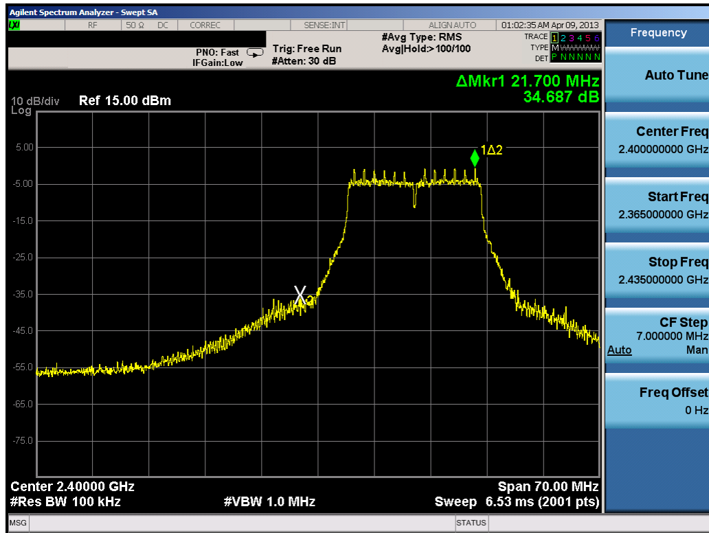
Plot 6-27. Band Edge Plot (802.11g– Ch. 1)
