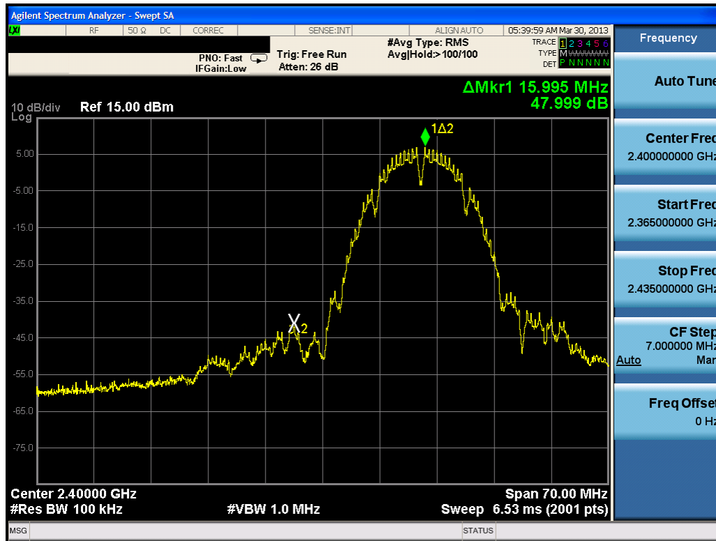
Plot 6-25. Band Edge Plot (802.11b – Ch. 1)
