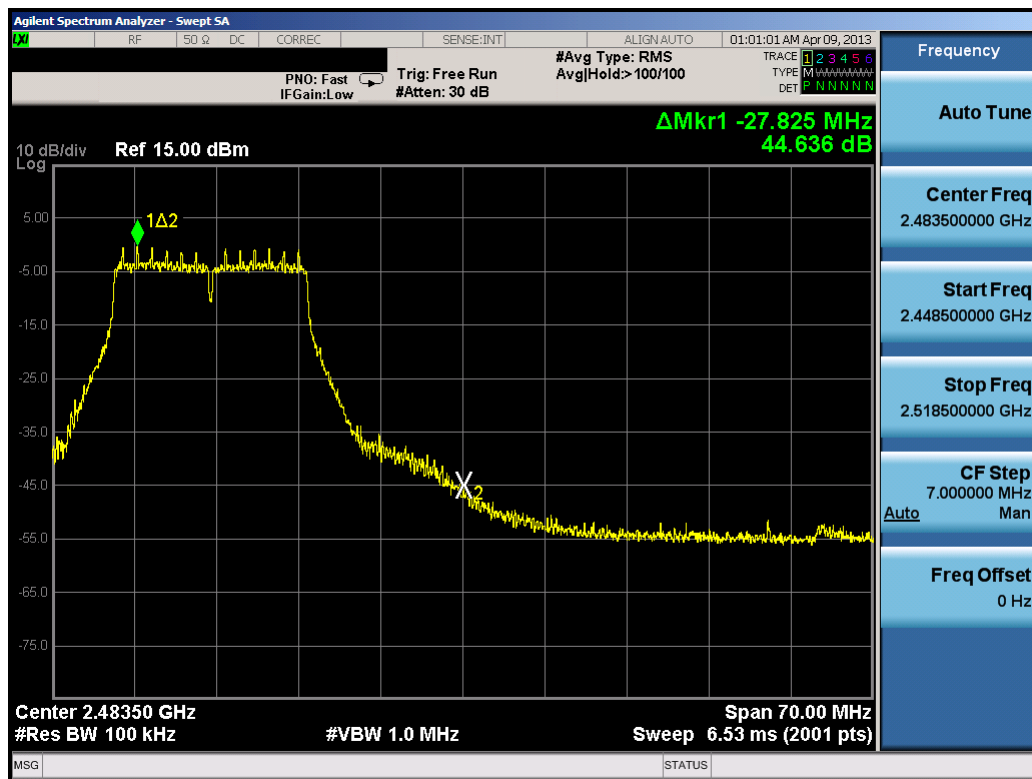
Plot 6-28. Band Edge Plot (802.11g – Ch. 11)
