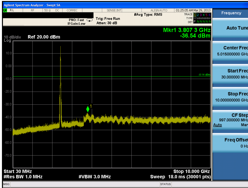
Plot 6-35. Conducted Spurious Plot (802.11b – Ch. 6)
