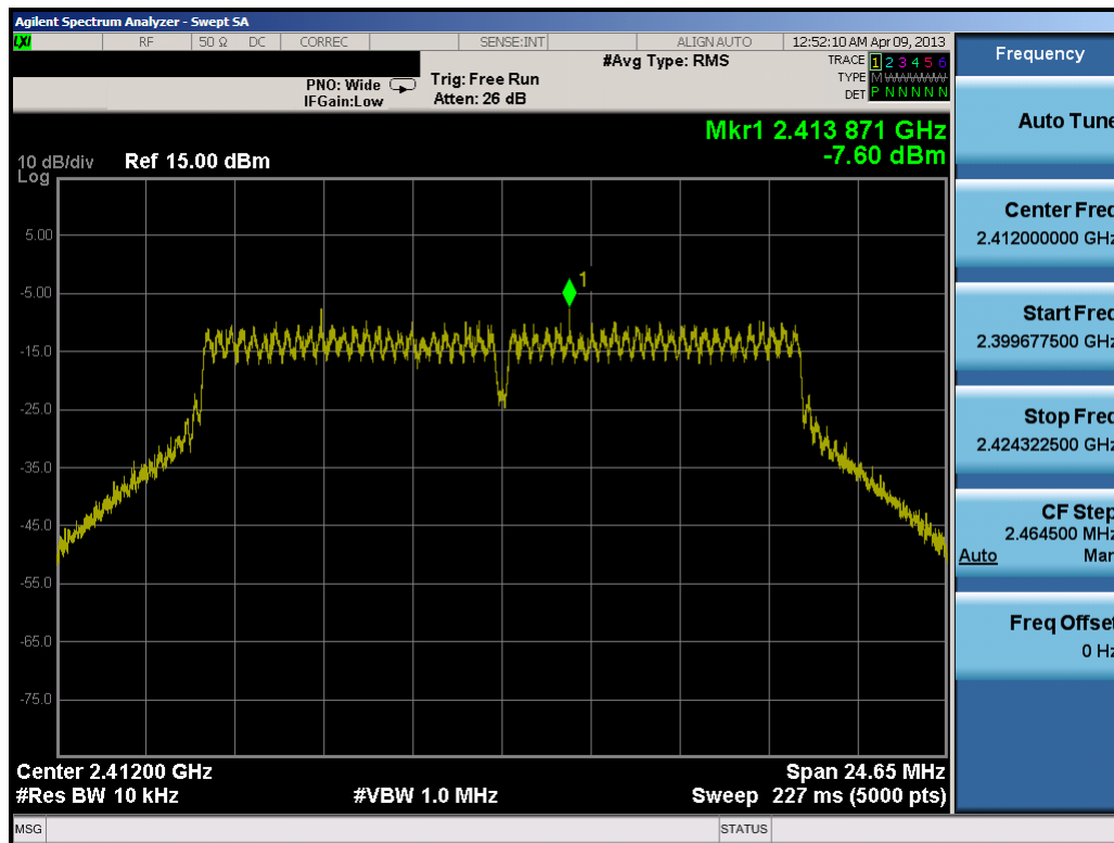
Plot 6-16. Power Spectral Density Plot (802.11g – Ch. 1)
