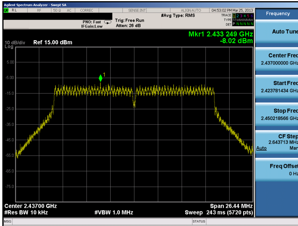
Plot 6-23. Power Spectral Density Plot (802.11n (2.4GHz – 800ns GI) – Ch. 6)
