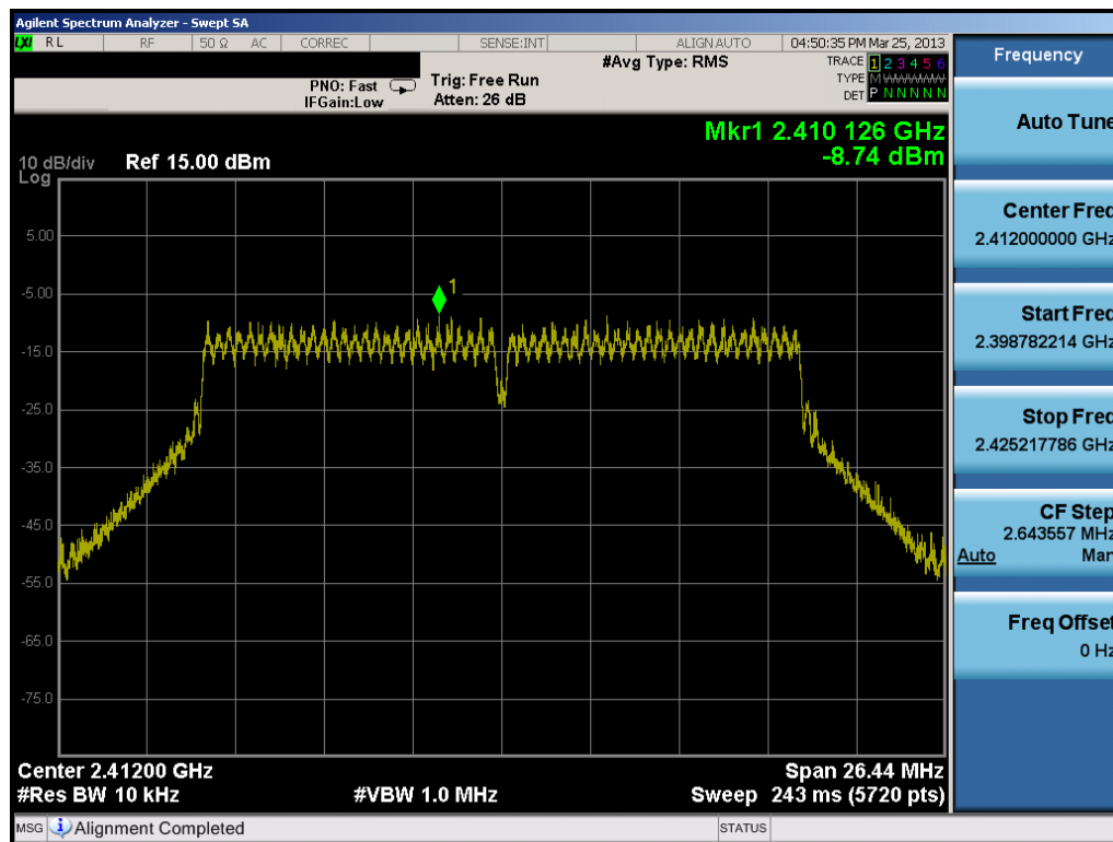
Plot 6-22. Power Spectral Density Plot (802.11n (2.4GHz – 800ns GI) – Ch. 1)
