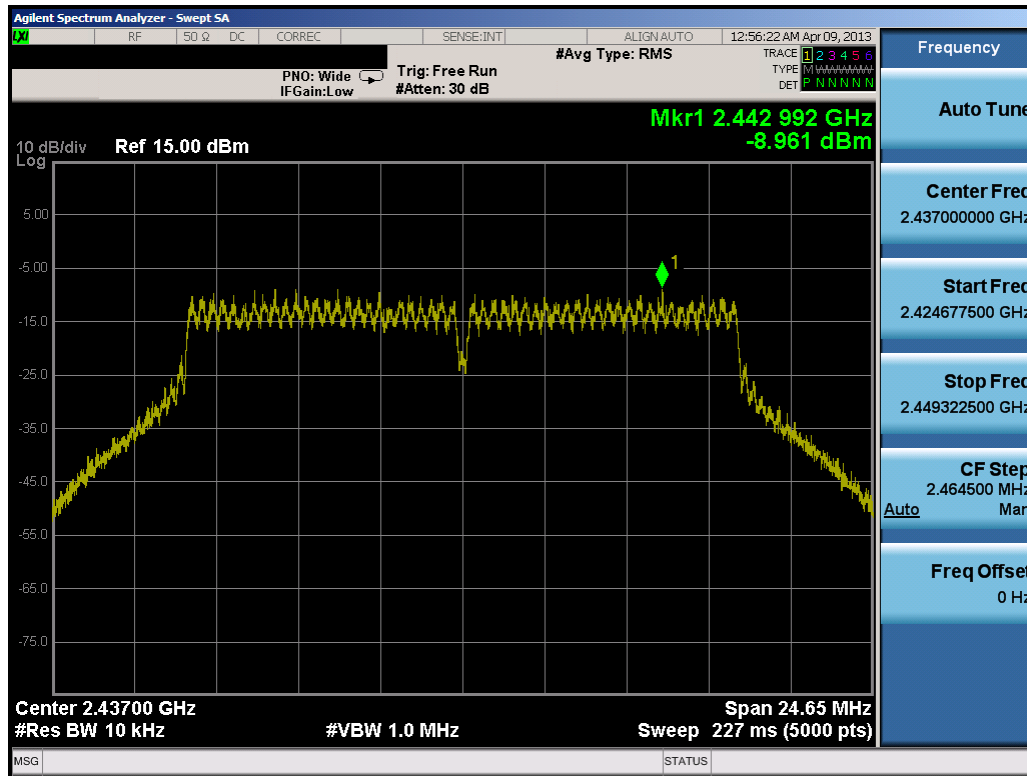
Plot 6-17. Power Spectral Density Plot (802.11g – Ch. 6)
