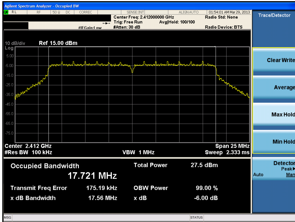
Plot 6-7. 6dB Bandwidth Plot (802.11n (2.4GHz – 400ns GI) – Ch. 1)
