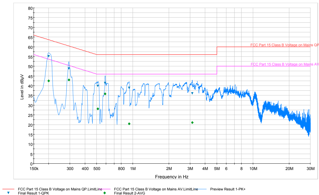
Plot 6-43. Line Conducted Plot with 802.11b (L1)
