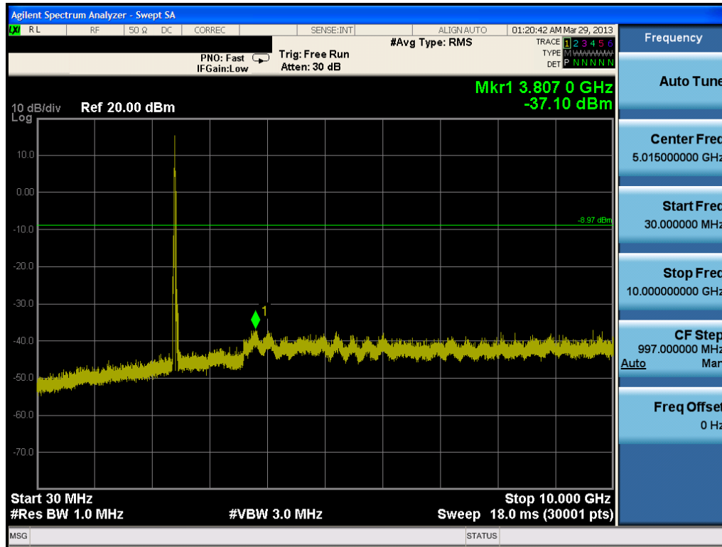
Plot 6-33. Conducted Spurious Plot (802.11b – Ch. 1)
