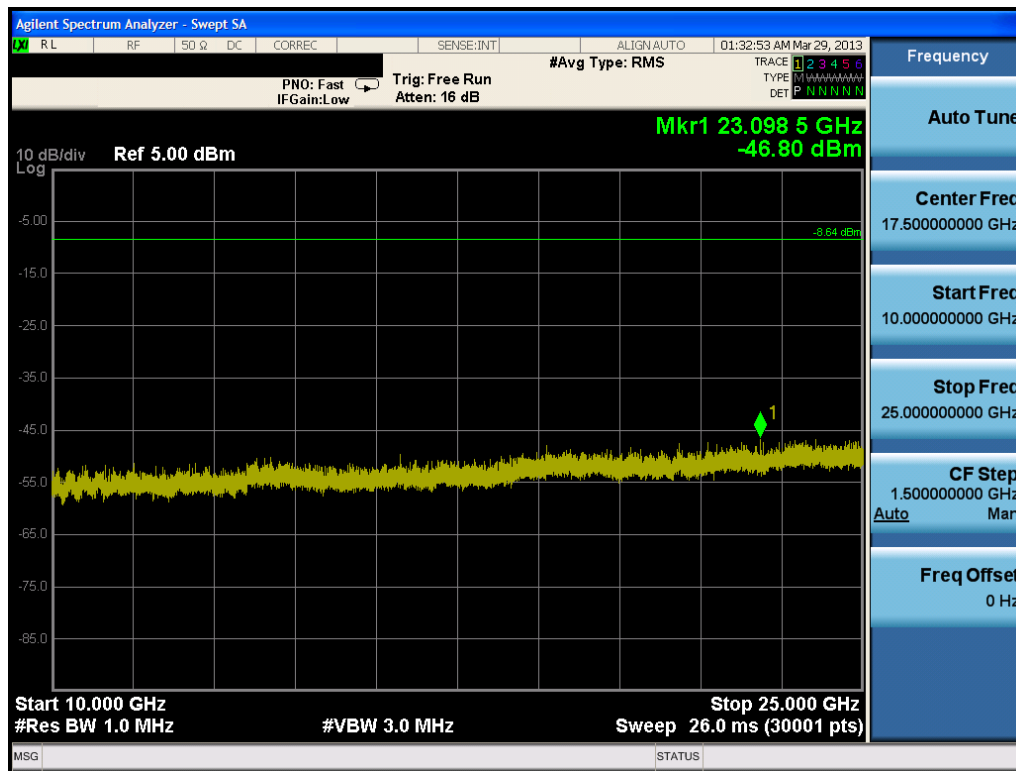
Plot 6-38. Conducted Spurious Plot (802.11b – Ch. 11)
