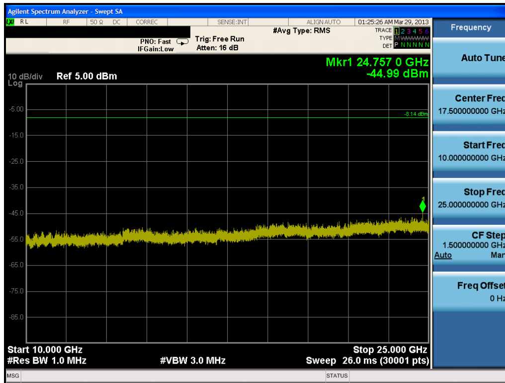
Plot 6-36. Conducted Spurious Plot (802.11b – Ch. 6)
