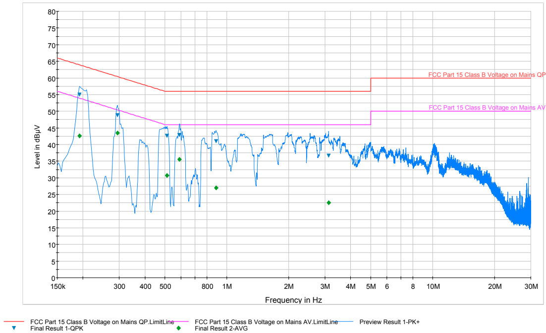
Plot 6-44. Line Conducted Plot with 802.11b (N)
