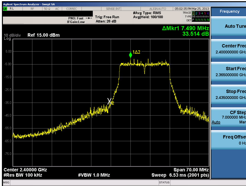
Plot 6-29. Band Edge Plot (802.11n (2.4GHz – 400ns GI) – Ch. 1)
