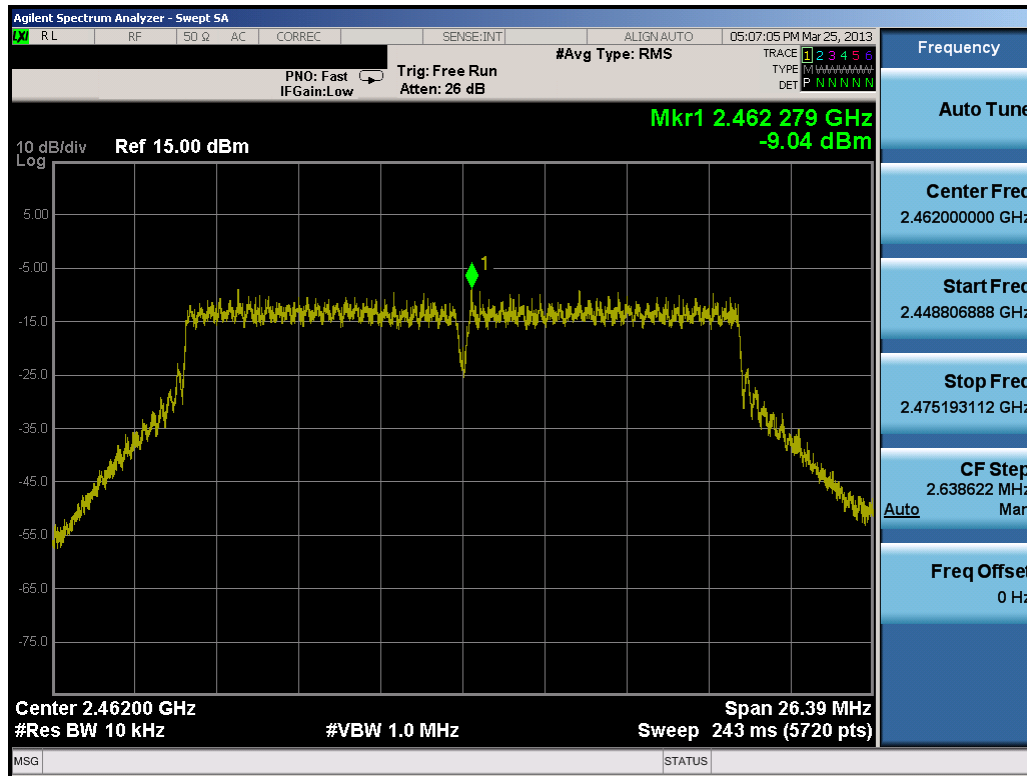
Plot 6-21. Power Spectral Density Plot (802.11n (2.4GHz – 400ns GI) – Ch. 11)
