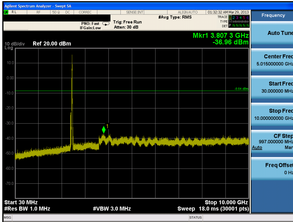
Plot 6-37. Conducted Spurious Plot (802.11b – Ch. 11)
