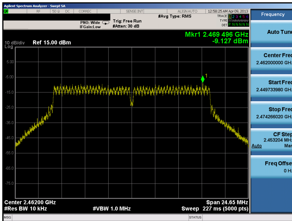
Plot 6-18. Power Spectral Density Plot (802.11g – Ch. 11)
