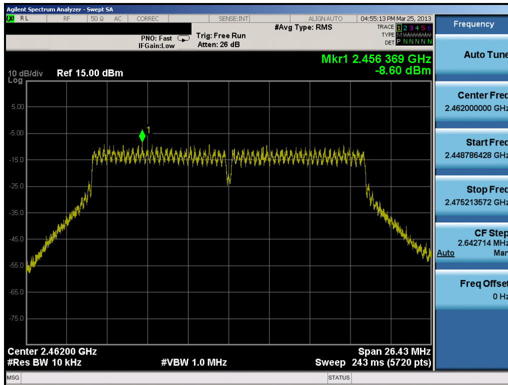
Plot 6-24. Power Spectral Density Plot (802.11n (2.4GHz – 800ns GI) – Ch. 11)
