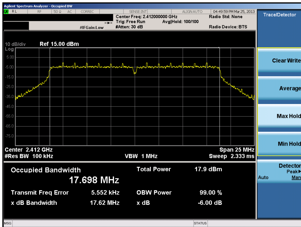
Plot 6-10. 6dB Bandwidth Plot (802.11n (2.4GHz – 800ns GI) – Ch. 1)
