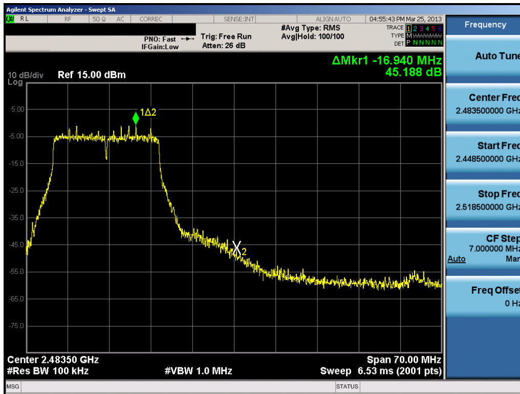
Plot 6-32. Band Edge Plot (802.11n (2.4GHz – 800ns GI) – Ch. 11)
