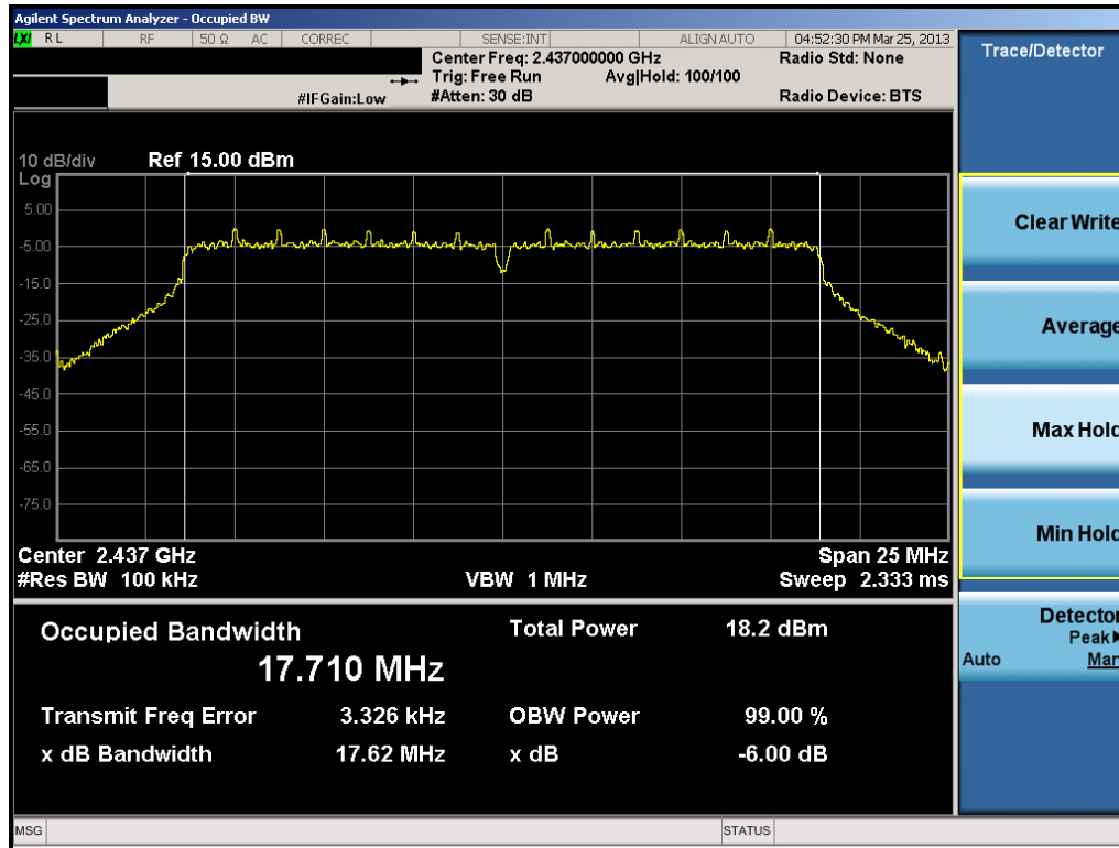
Plot 6-11. 6dB Bandwidth Plot (802.11n (2.4GHz – 800ns GI) – Ch. 6)
