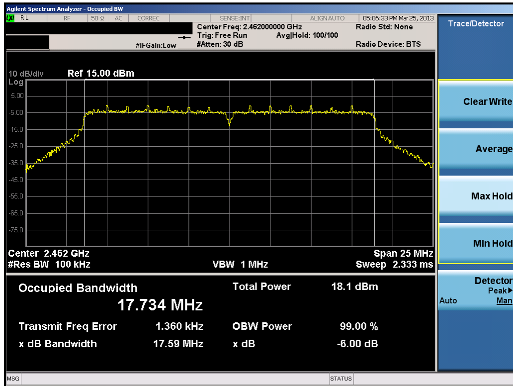
Plot 6-9. 6dB Bandwidth Plot (802.11n (2.4GHz – 400ns GI) – Ch. 11)
