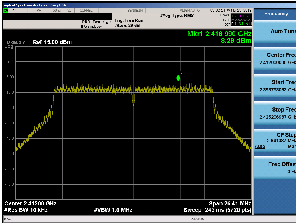
Plot 6-19. Power Spectral Density Plot (802.11n (2.4GHz – 400ns GI) – Ch. 1)
