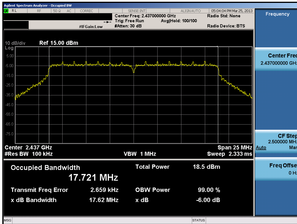
Plot 6-8. 6dB Bandwidth Plot (802.11n (2.4GHz – 400ns GI) – Ch. 6)
