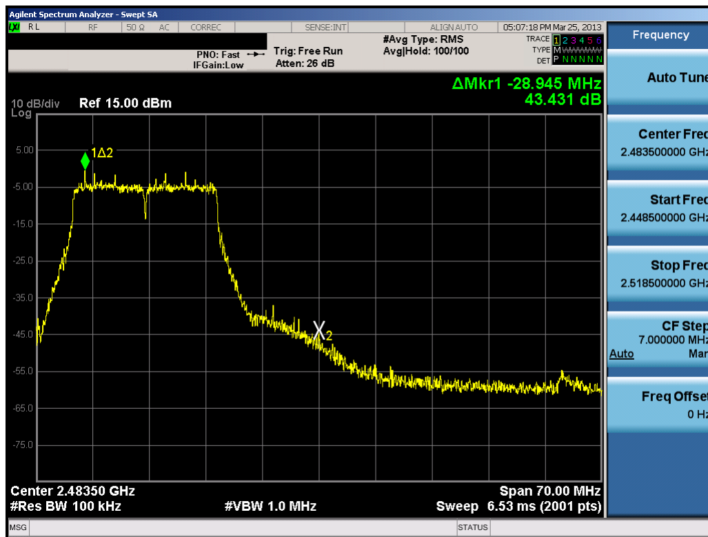
Plot 6-30. Band Edge Plot (802.11n (2.4GHz – 400ns GI) – Ch. 11)
