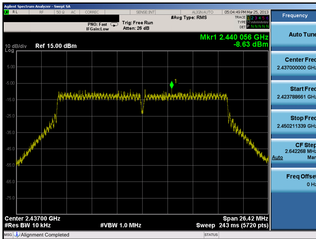
Plot 6-20. Power Spectral Density Plot (802.11n (2.4GHz – 400ns GI) – Ch. 6)
