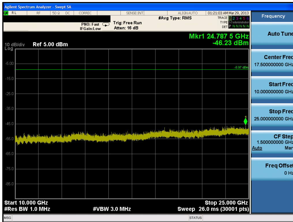
Plot 6-34. Conducted Spurious Plot (802.11b – Ch. 1)
