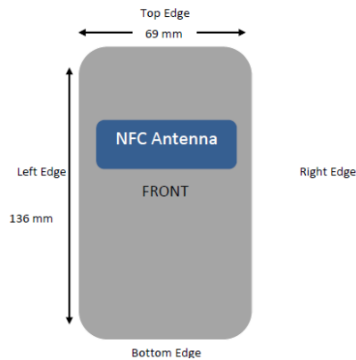
Figure 1-1 NFC Antenna Locations
