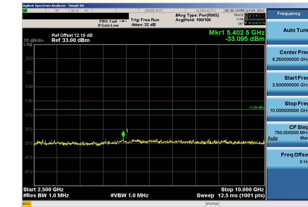
Plot 7-21. Conducted Spurious Plot (Cellular WCDMA Mode – Ch. 4132)
