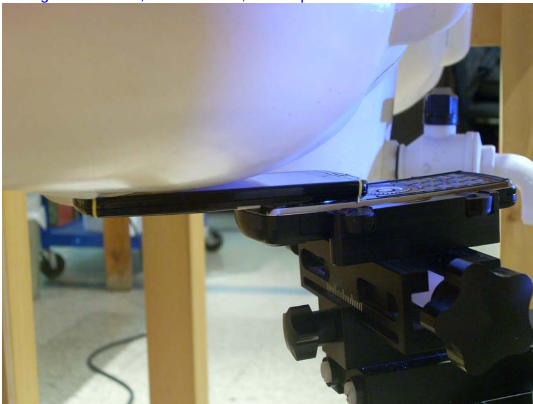
5. Right Head SAR, Cheek Touch, Slide Up
