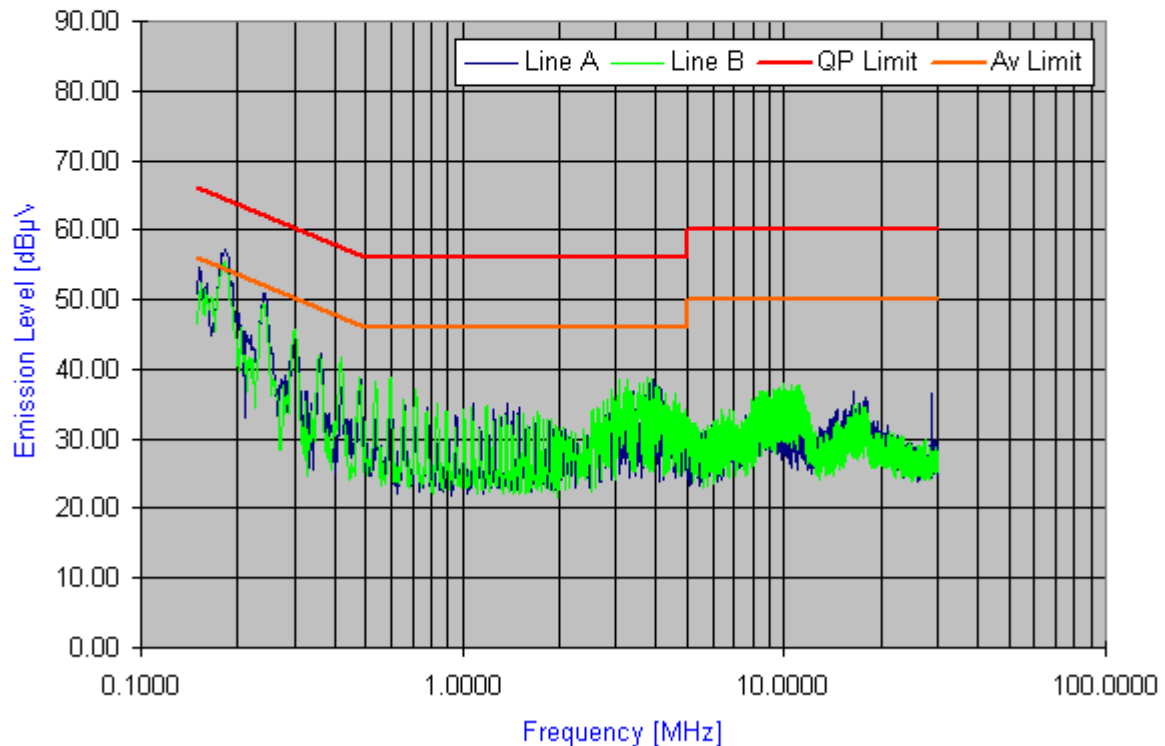
Plot 7-1. Line-Conducted Test Plot
