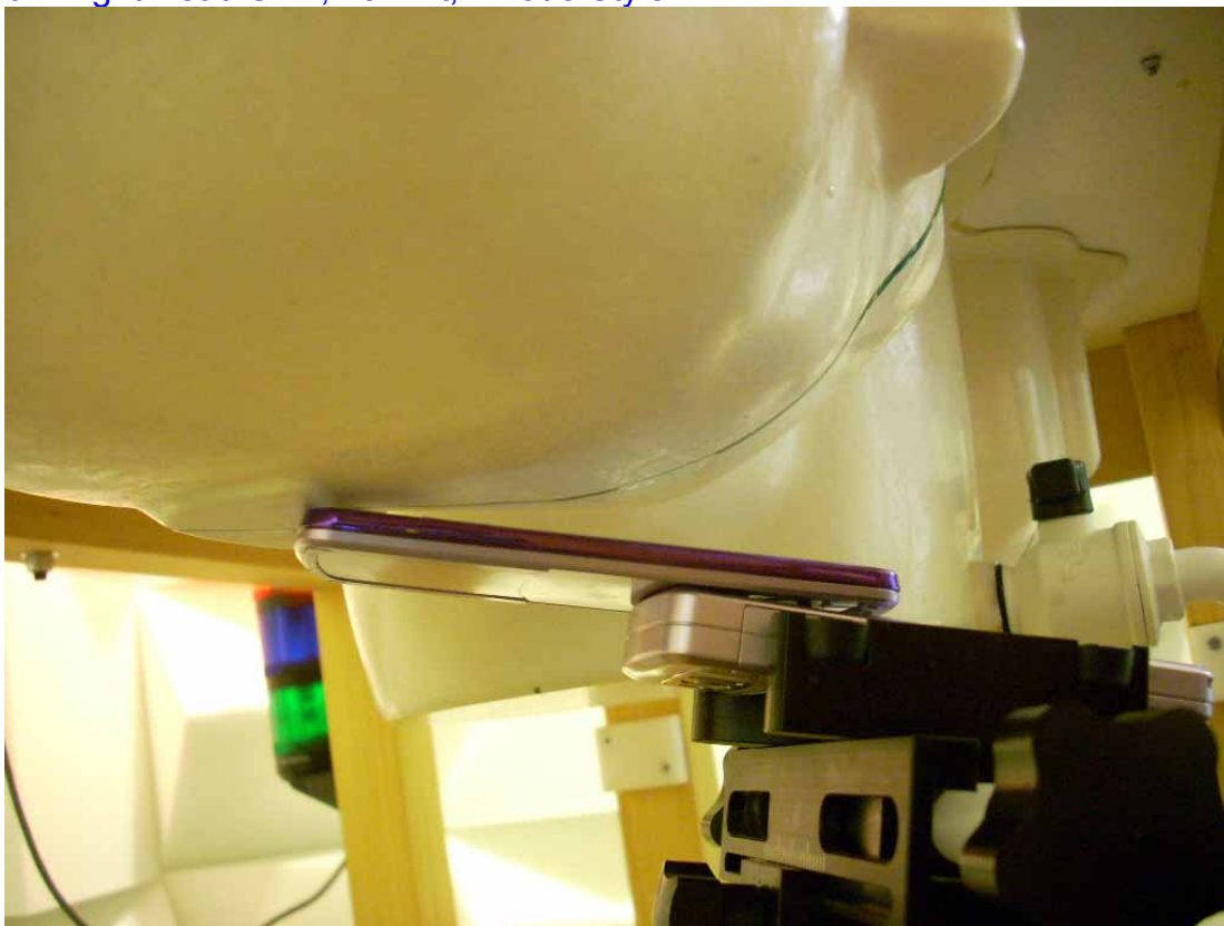
6. Right Head SAR, 15° Tilt, i-mode Style.
