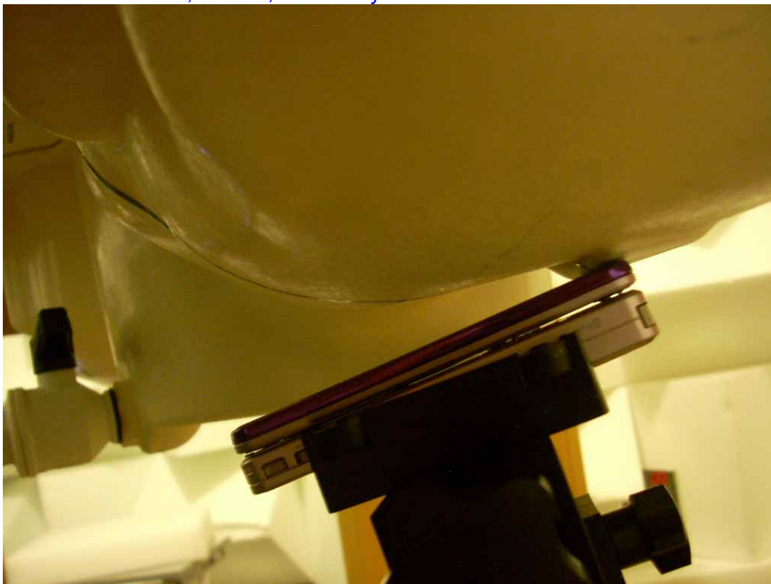
10. Left Head SAR, 15° Tilt, i-mode Style
