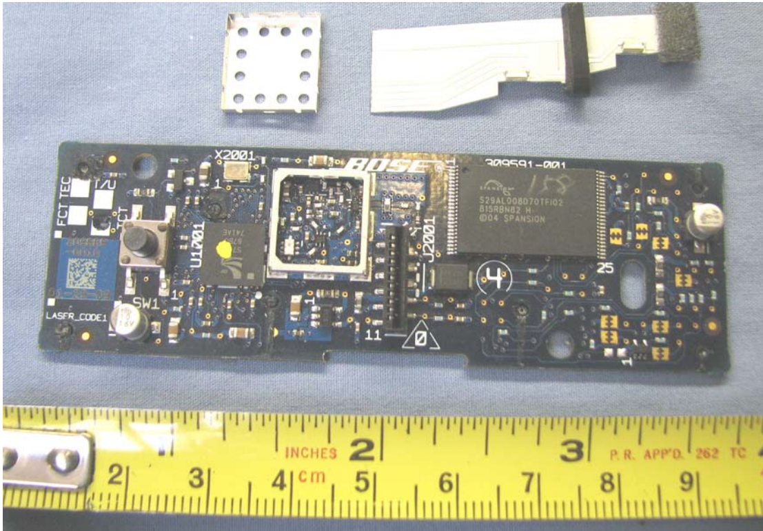
Top view of board – shield can and antenna removed
