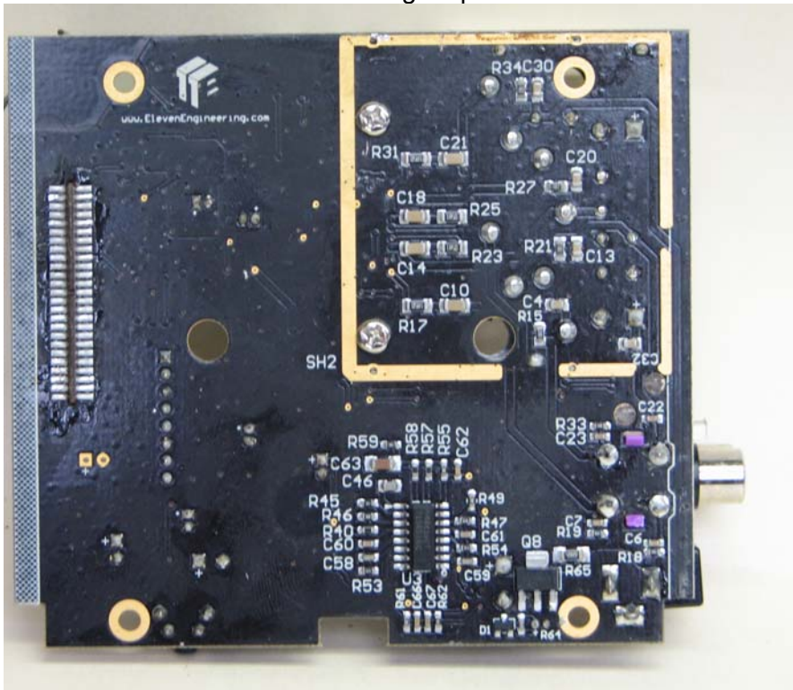
Shield cover for the audio switching amp removed
