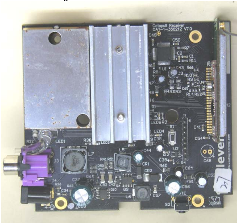
Shield cover for the audio switching amp removed
