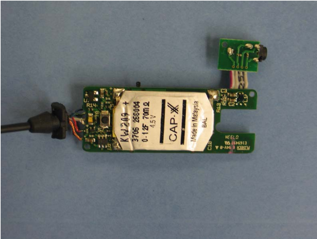
Board side 2, connector board removed
