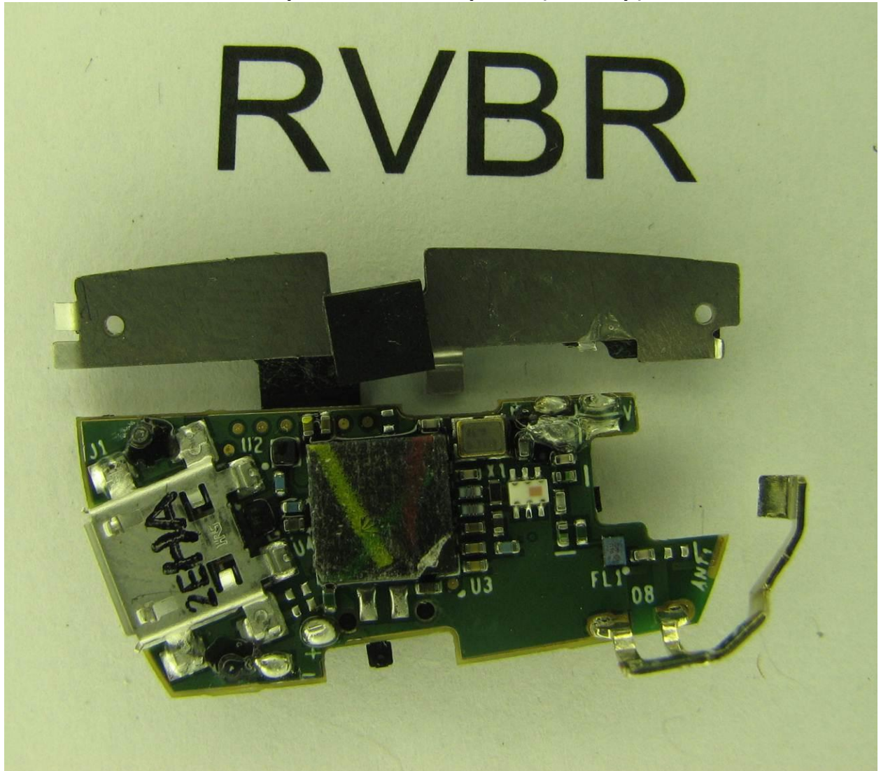
Component side PCB photo (close up)
