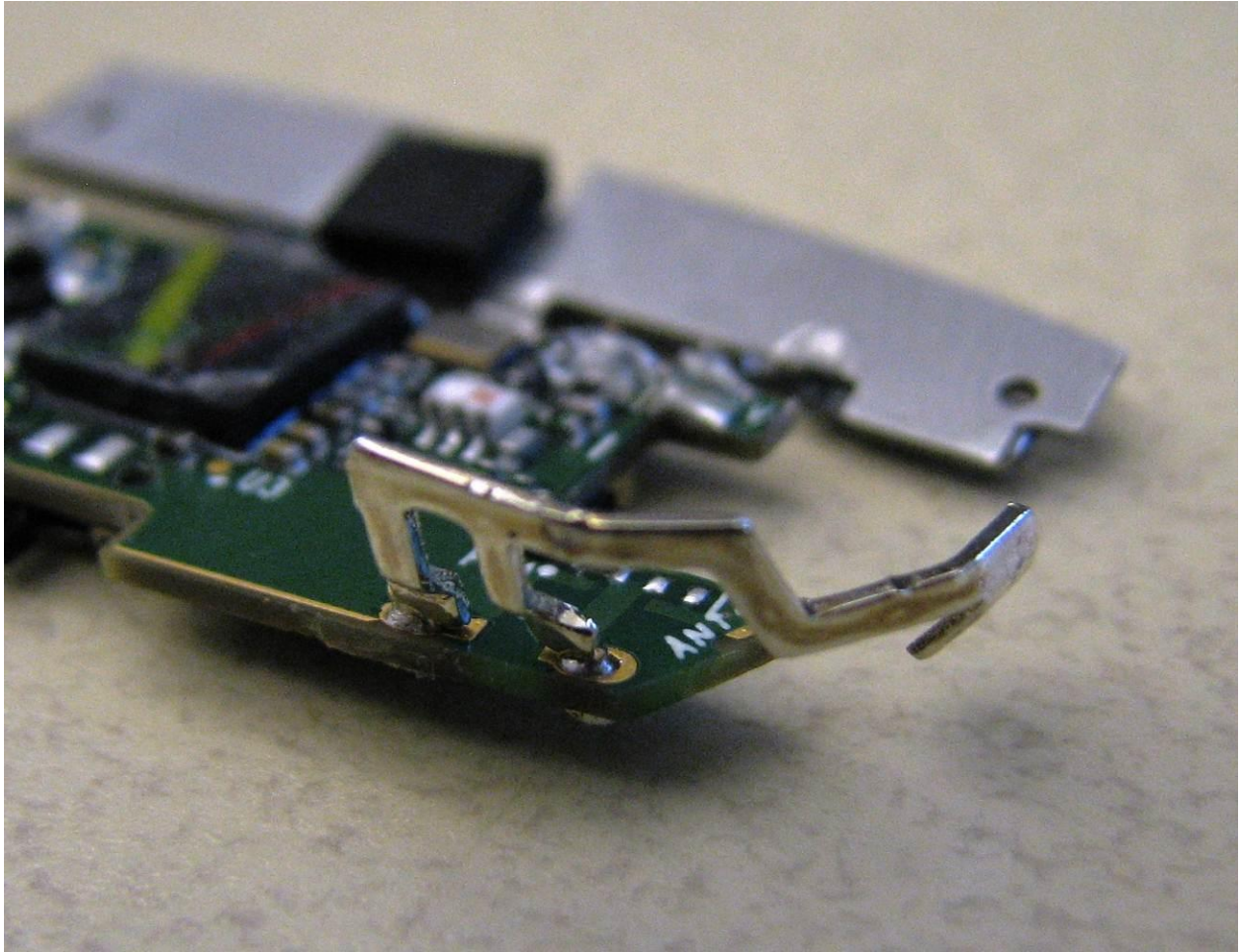
Antenna close up photo
