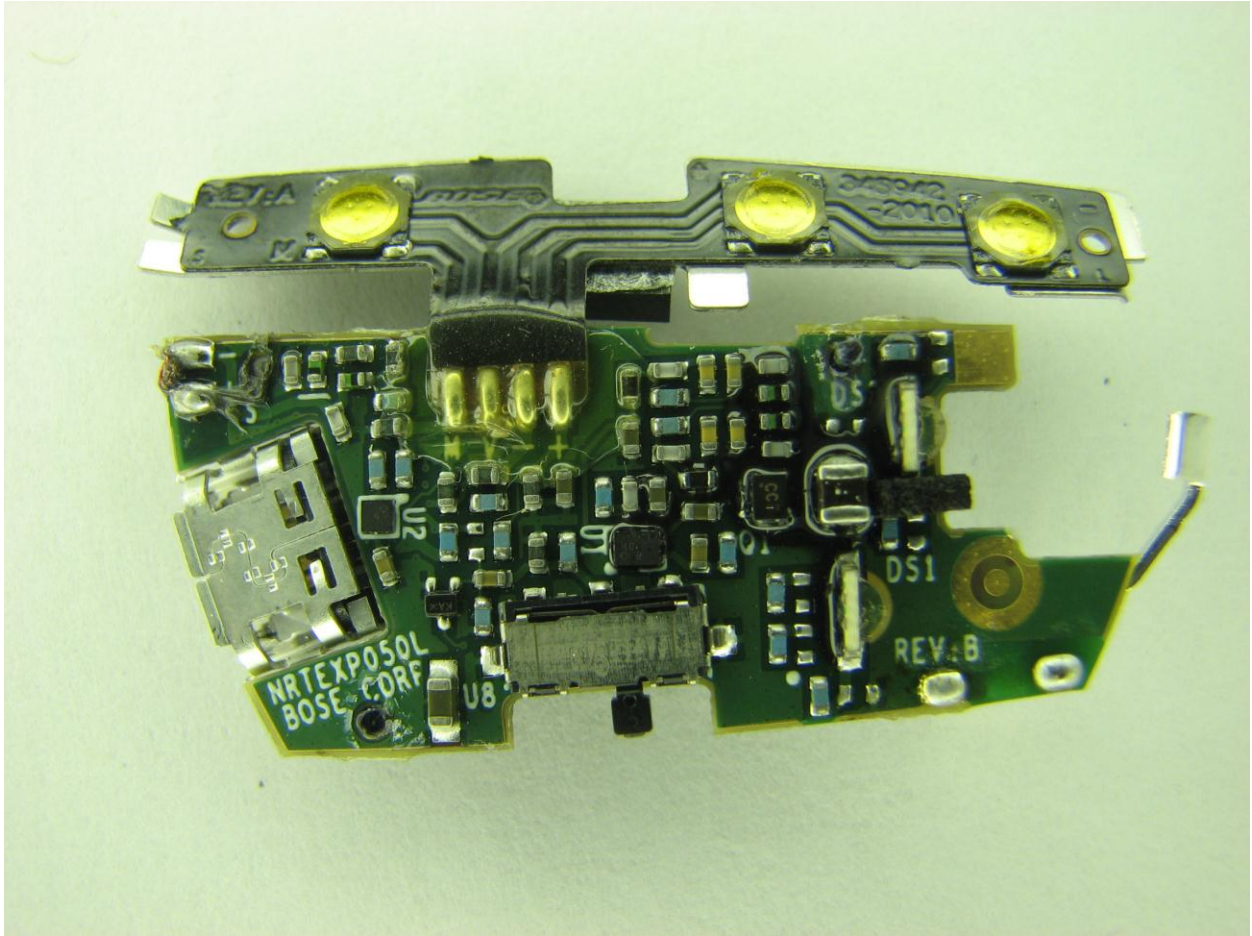
Bottom side PCB photo.
