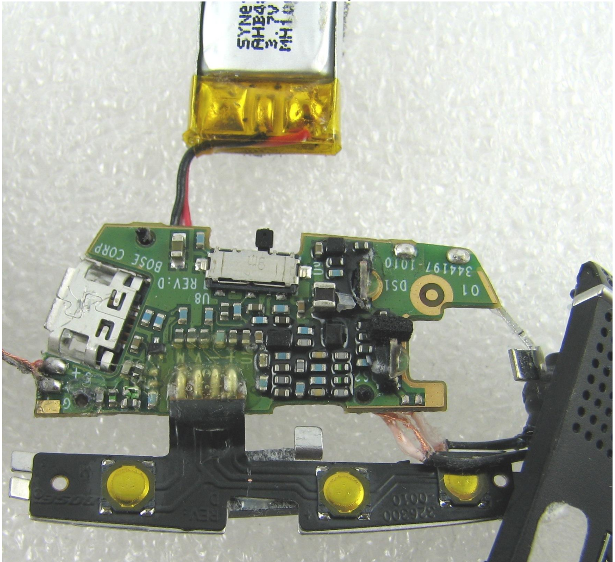
Bottom side PCB photo.
