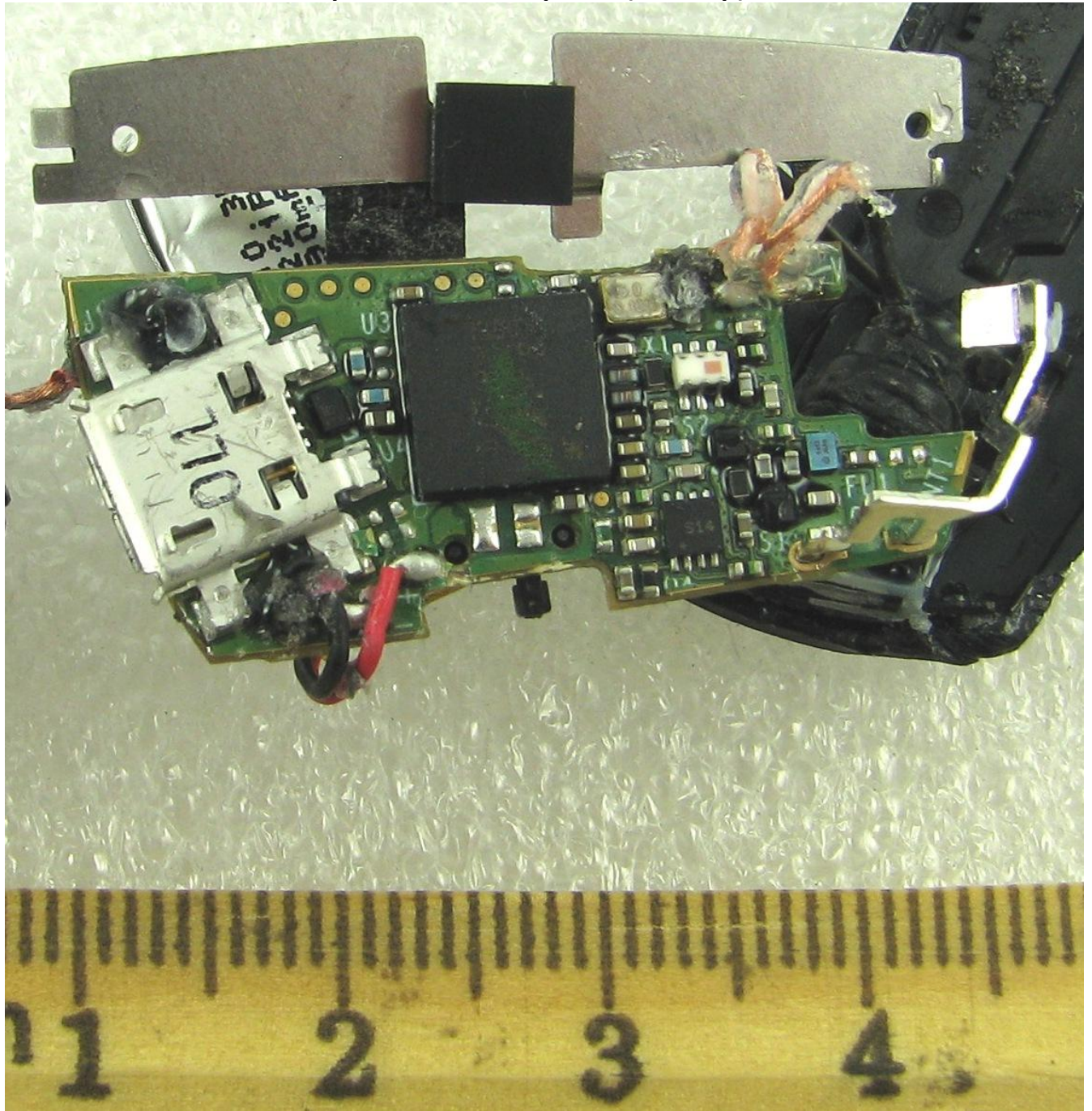
Component side PCB photo (close up)
