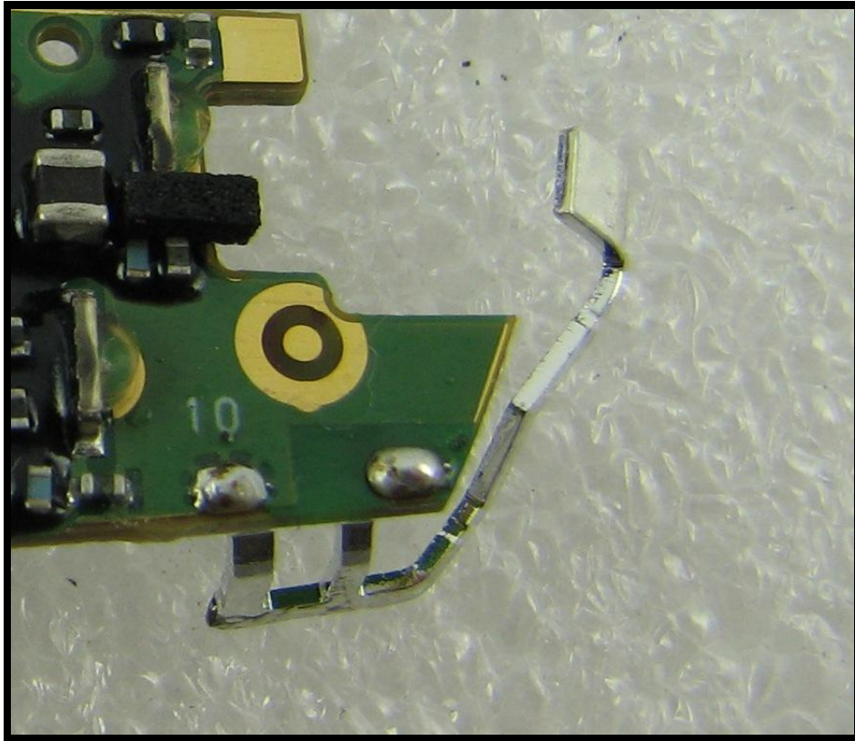
Antenna close up photo
