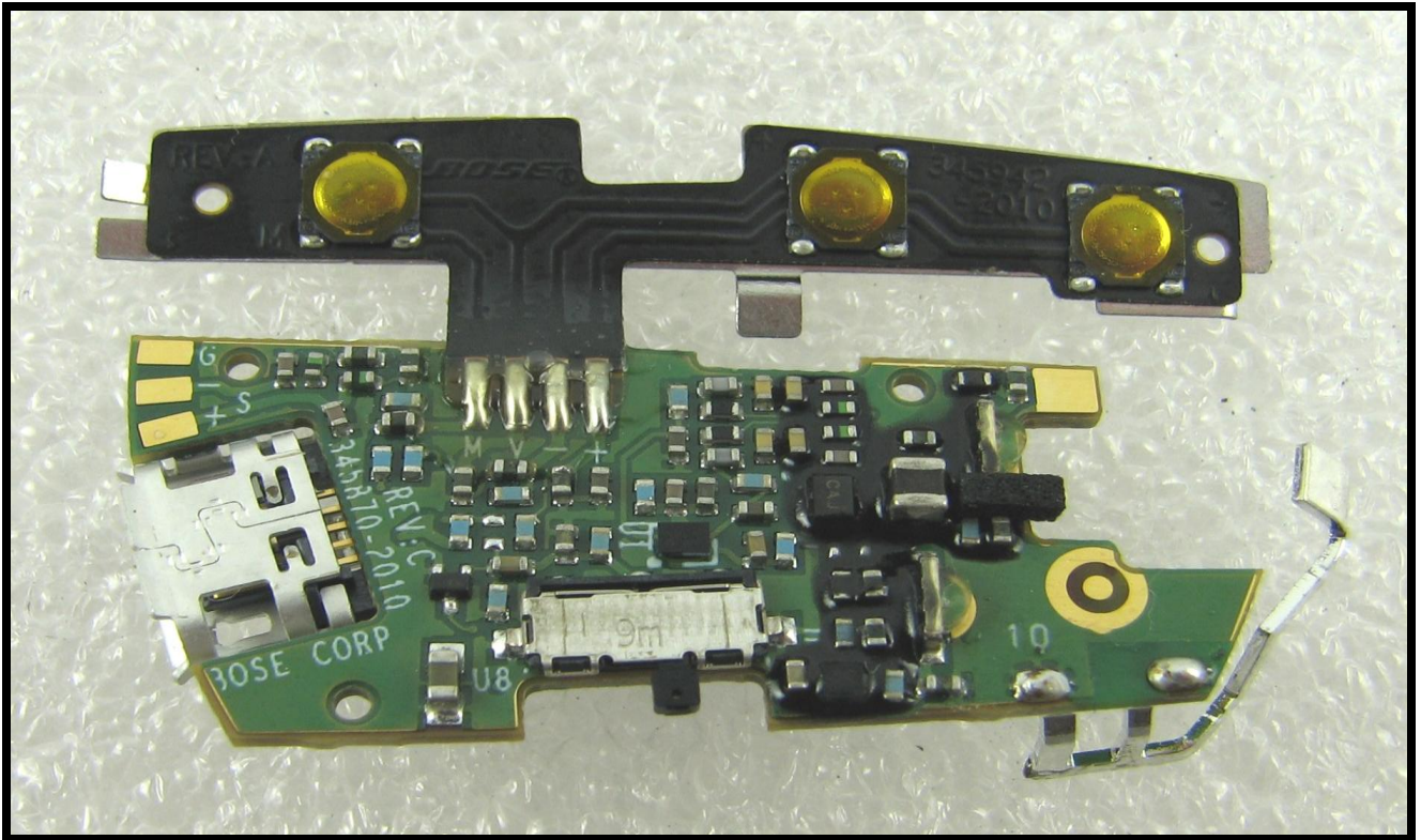
Bottom side PCB photo.
