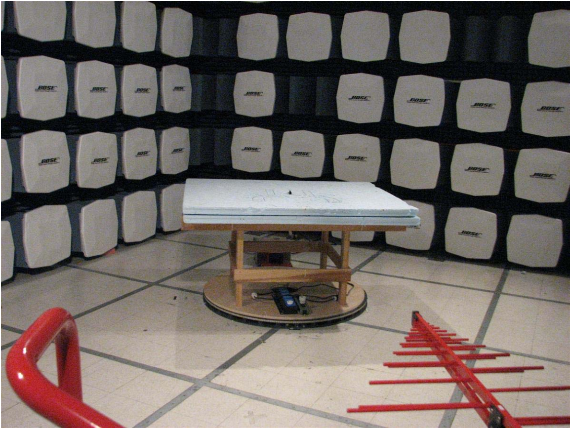
Test setup photos Radiated emissions – 30MHz – 4GHz
