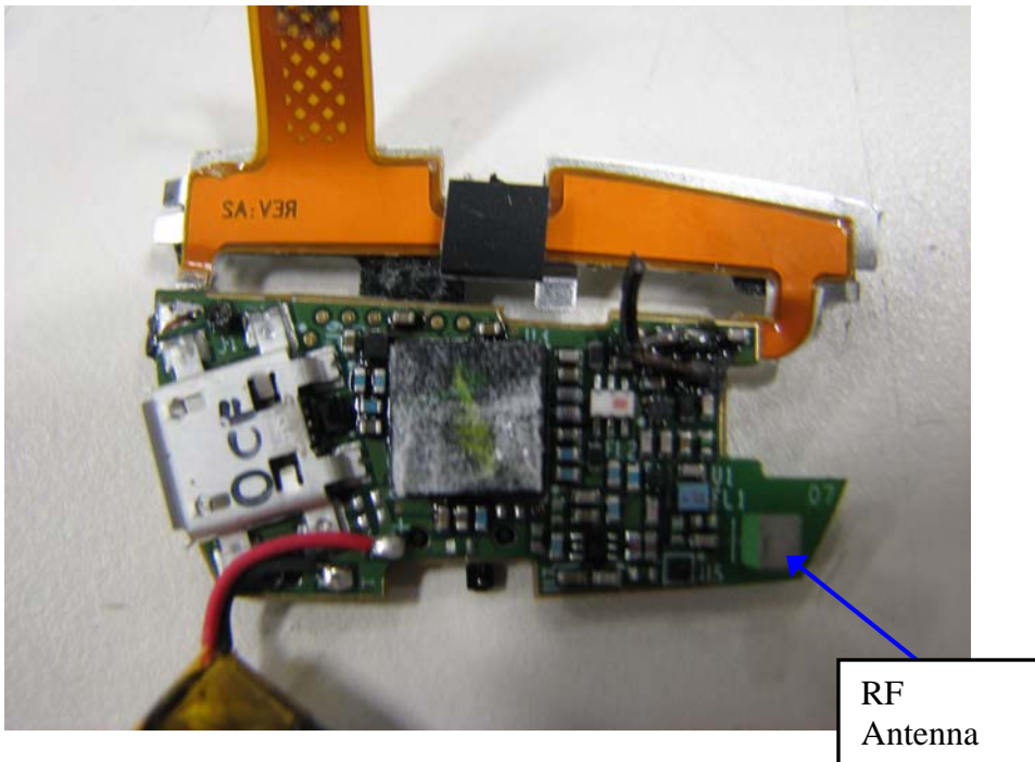
Internal PCB photo – close up of top side
