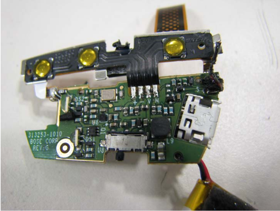
Internal PCB photo- bottom side
