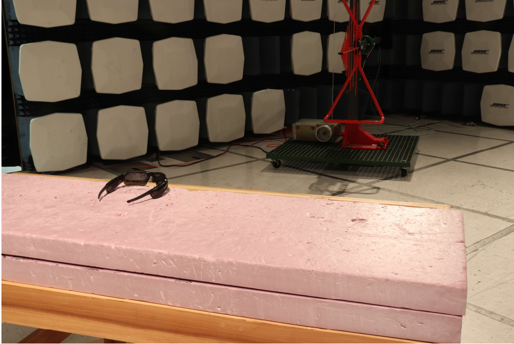
Radiated Emissions 30 MHz to 1 GHz, normal operation
