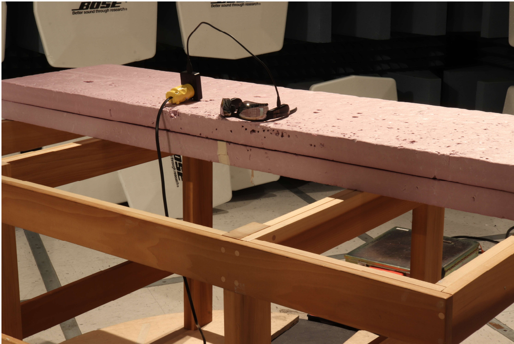
Radiated Emissions 30 MHz to 1 GHz, charging
