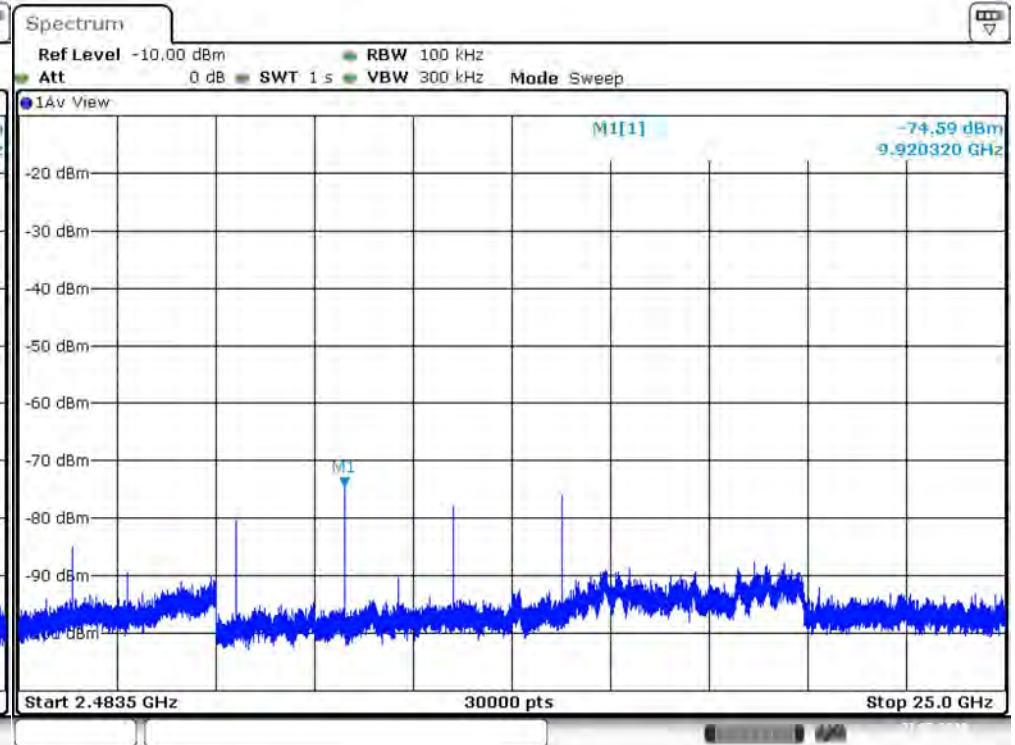
Plot2 DH5 2480 MHz Average Band 2
