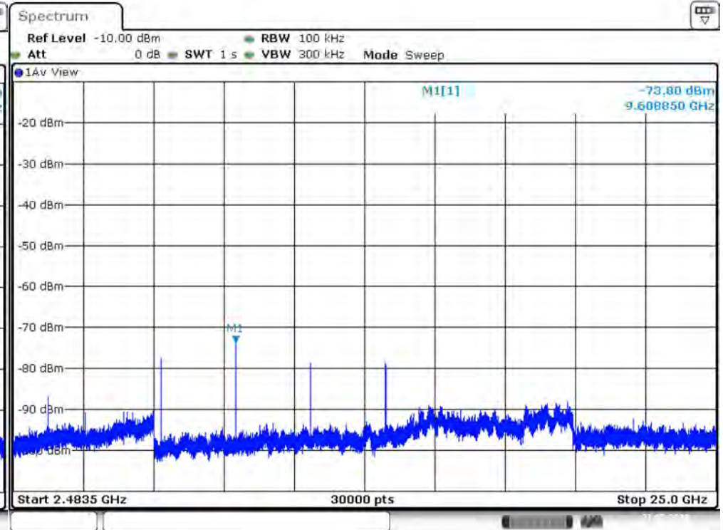
Plot2 DH5 2402 MHz Average Band 2
