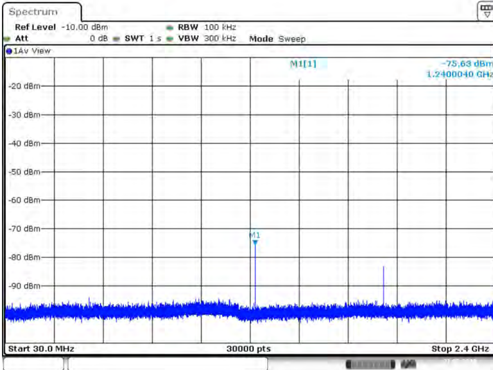
Plot1 DH5 2480 MHz Average Band 1
