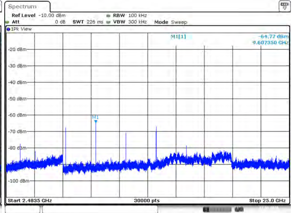
Plot2 DH5 2402 MHz Peak Band 2
