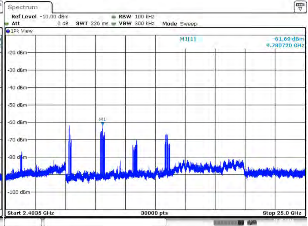
Plot2 DH5 Hopping Peak Band 2
