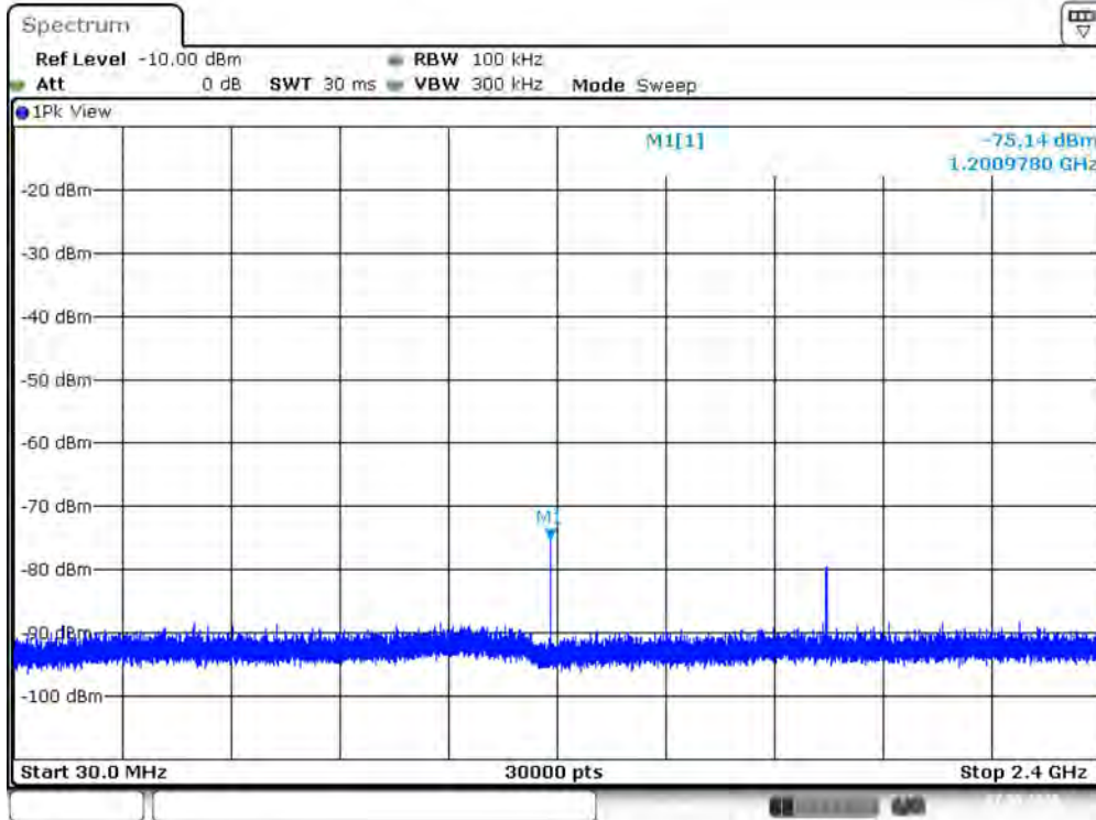
Plot1 DH5 2402 MHz Peak Band 1
