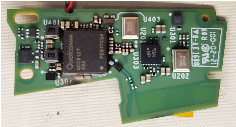
Main Board Bottom
