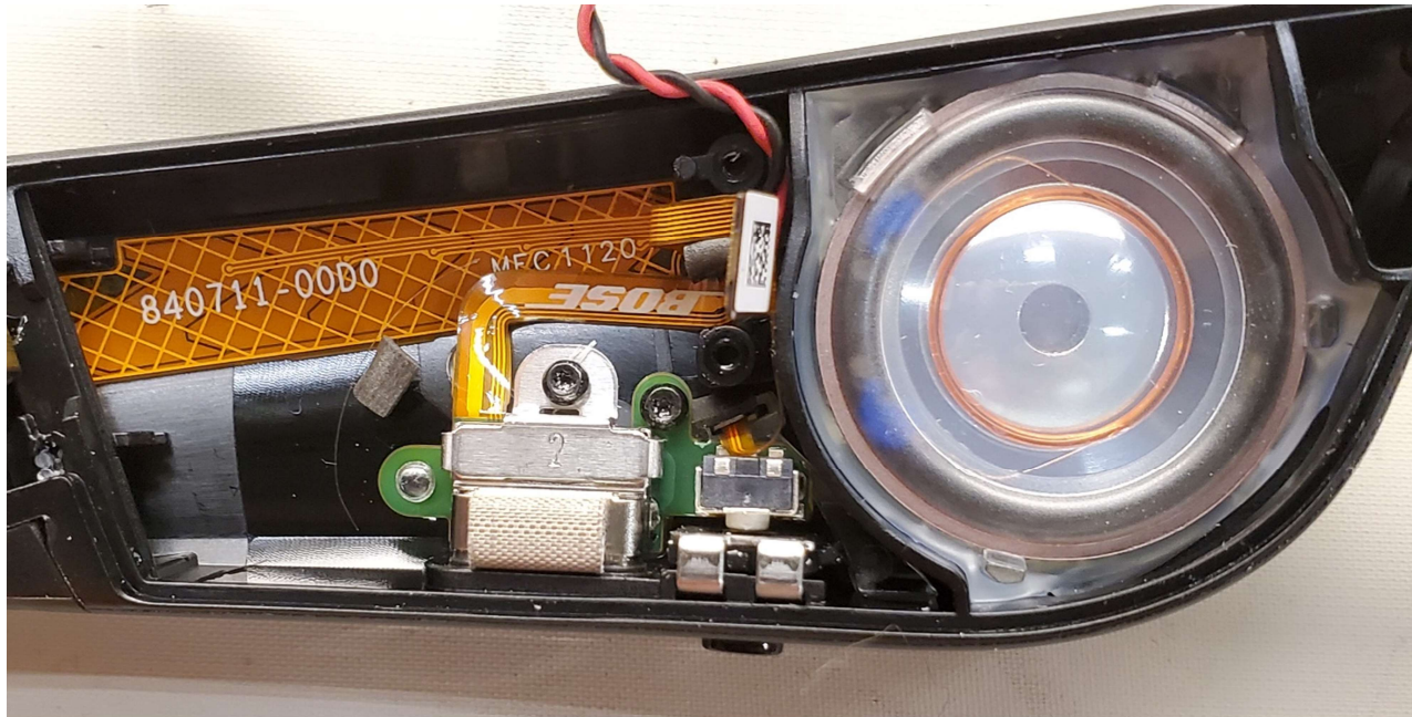
USB/LED & Capsense FPCs and transducer, Right temple
