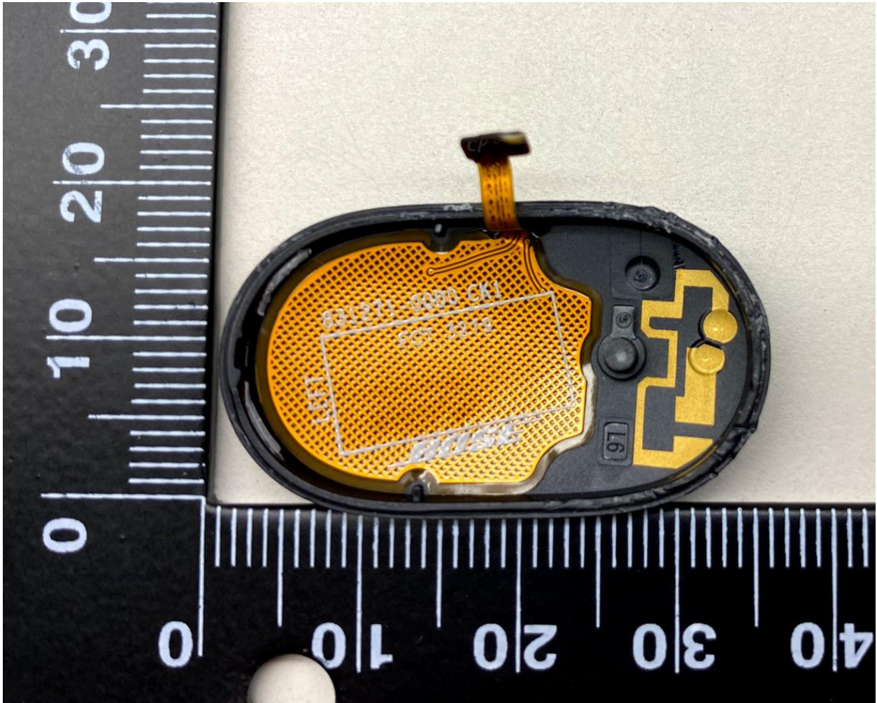
Bose Model BL3L Internal Photos
