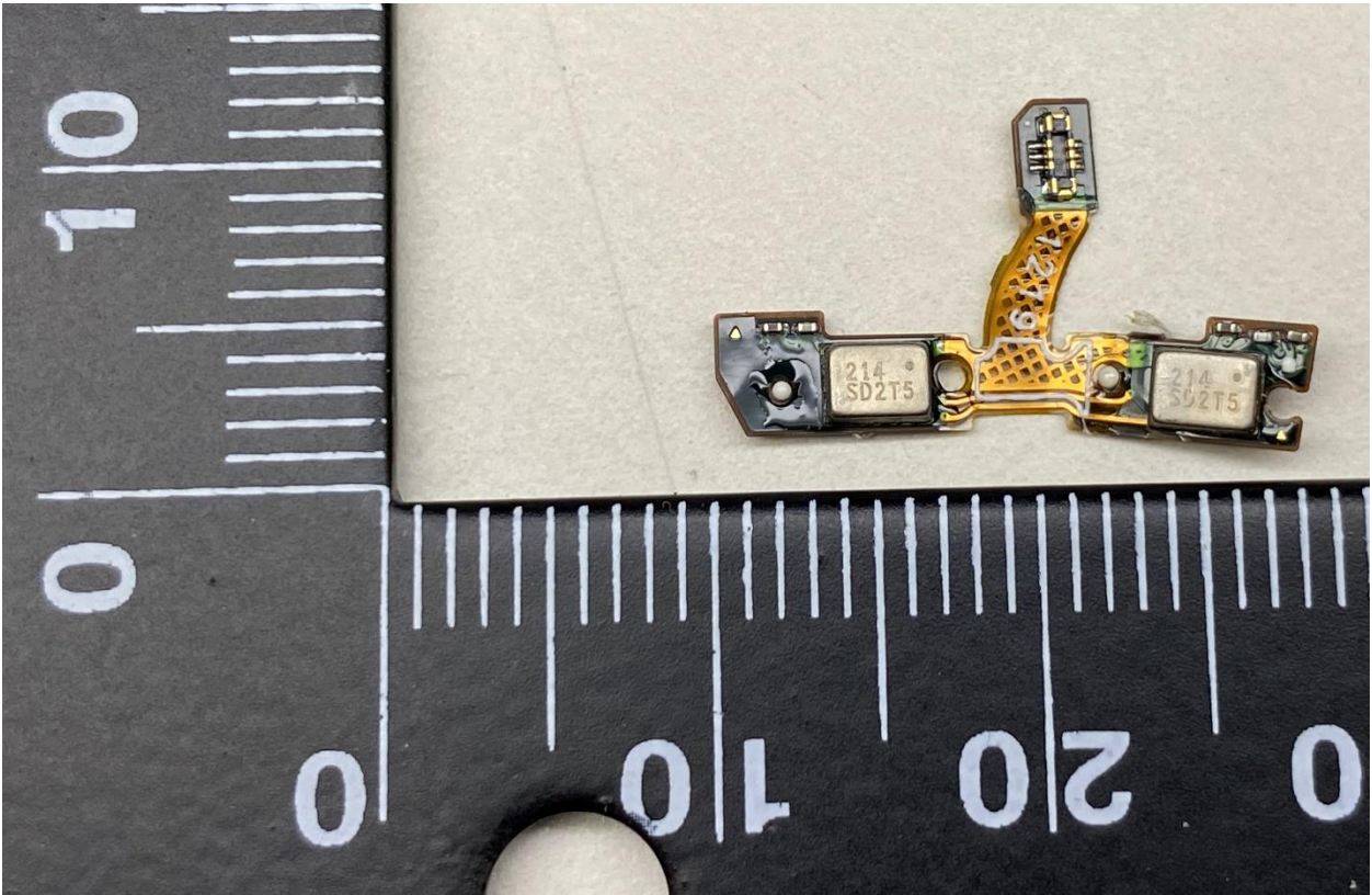
Bose Model BL3L Internal Photos
