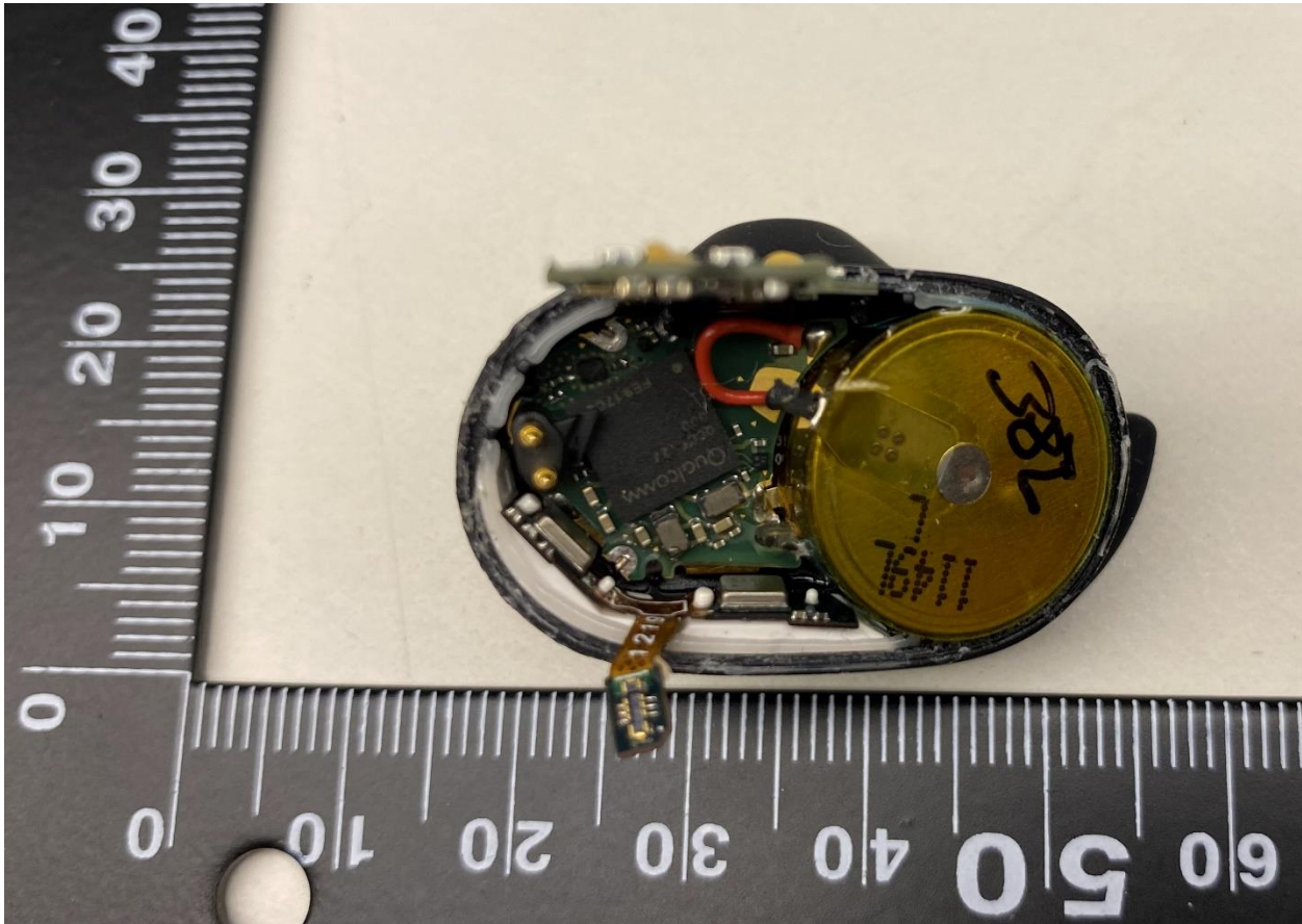
Bose Model BL3L Internal Photos
