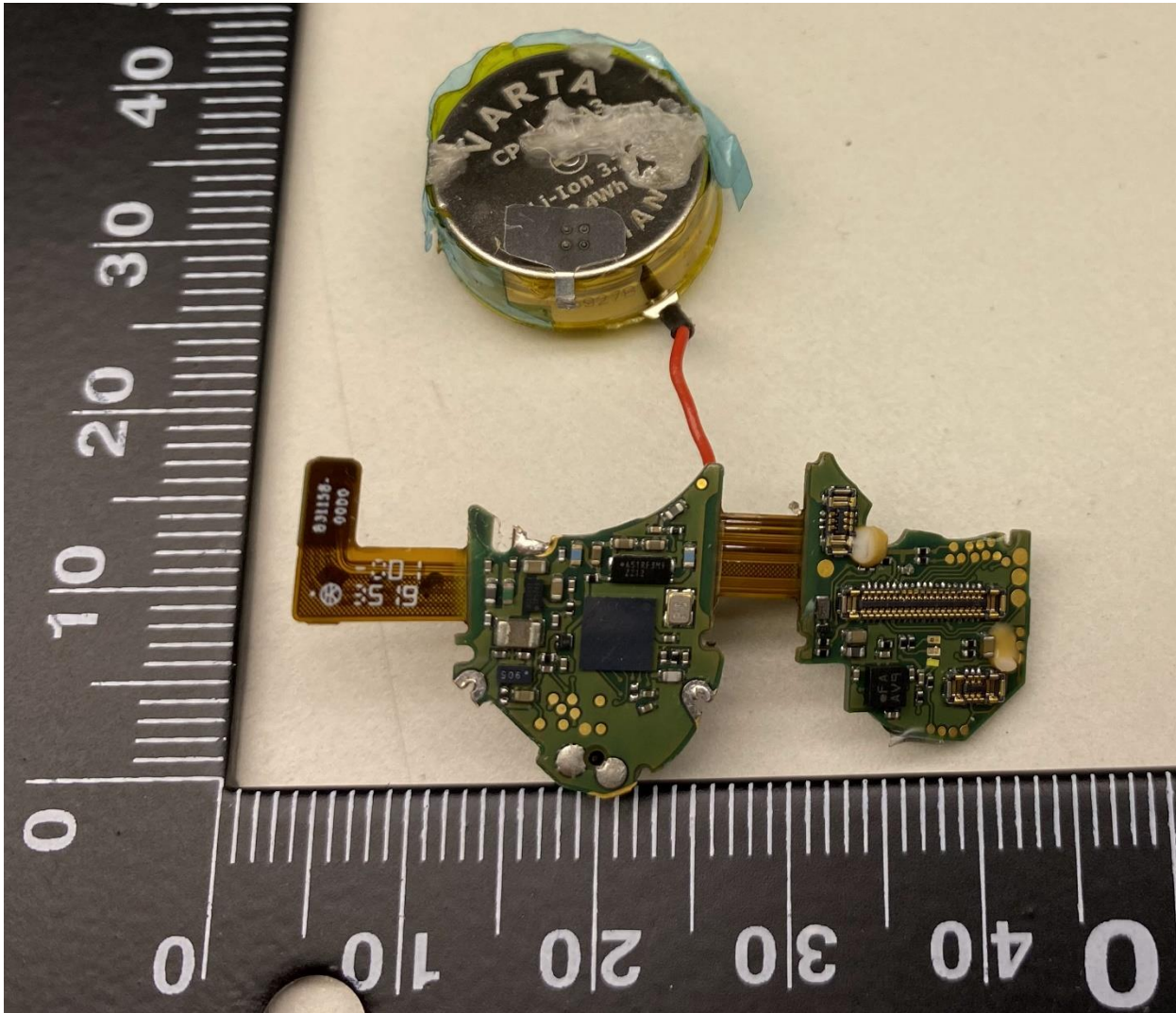
Bose Model BL3L Internal Photos
