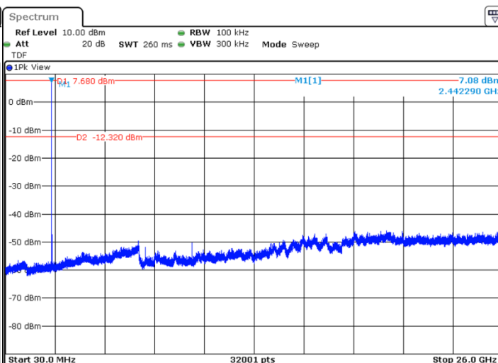
OUT-OF-BAND MID CHANNEL (2442MHz)
